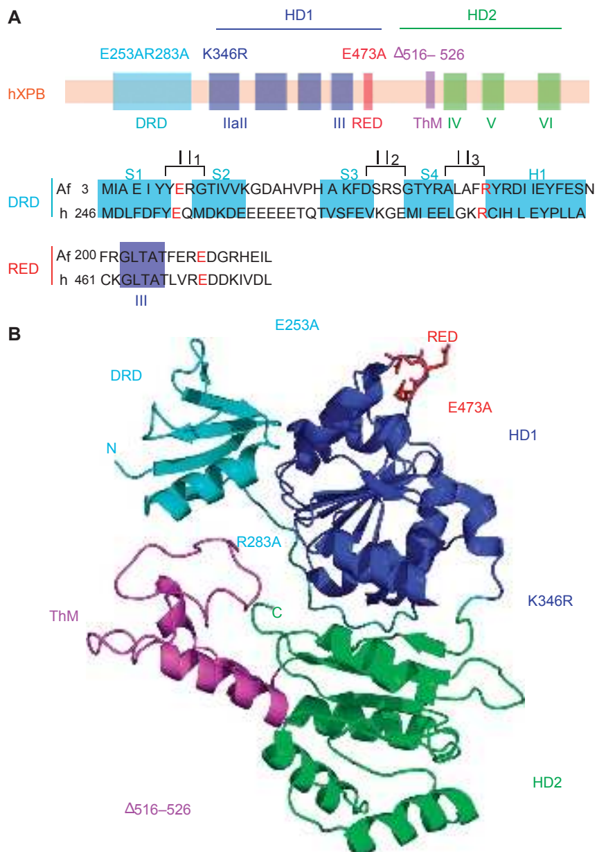
Figure 3 XPB conserved sequences, motifs and structural architecture (A) Upper panel shows the location of the human XPB structural domains: the four classical helicase motifs (I, Ia, II and III) of the first helicase module (HD1) are indicated in blue. The three helicase motifs (IV, V and VI) of the second helicase module (HD2) are indicated in green. The putative damage recognition (DRD), R-E-D and Thumb (ThM) domains identified in a homologue of XPB from the thermophilic organism Archaeoglobus fulgidus (Fanet al, 2006) are indicated, respectively in light blue, red and purple. The mutations E253A, R283A, K346R, E473A and \Delta 516–526 are annotated. Lower panel shows the sequence conservation of the DRD and R-E-D motifs between human (h) and Archaeoglobus fulgidus (Af) XPB proteins. The \alpha -strands (S1–4) and the \alpha -helix (H1) are indicated. Identical residues are marked in bold letters. The conserved helicase motif III indicated by a blue square is located close to the R-E-D motif indicated by a red open square. The three hairpin loops potentially involved in DNA binding are indicated (1, 2, 3). Residues mutated in this study are marked in red. (B) View of the ribbon representation of AfXPB. The HD1 is indicated in blue, HD2 in green. The putative DRD, R-E-D and ThM domains are indicated in light blue, red and purple, respectively. The positions of the new mutations are indicated.
