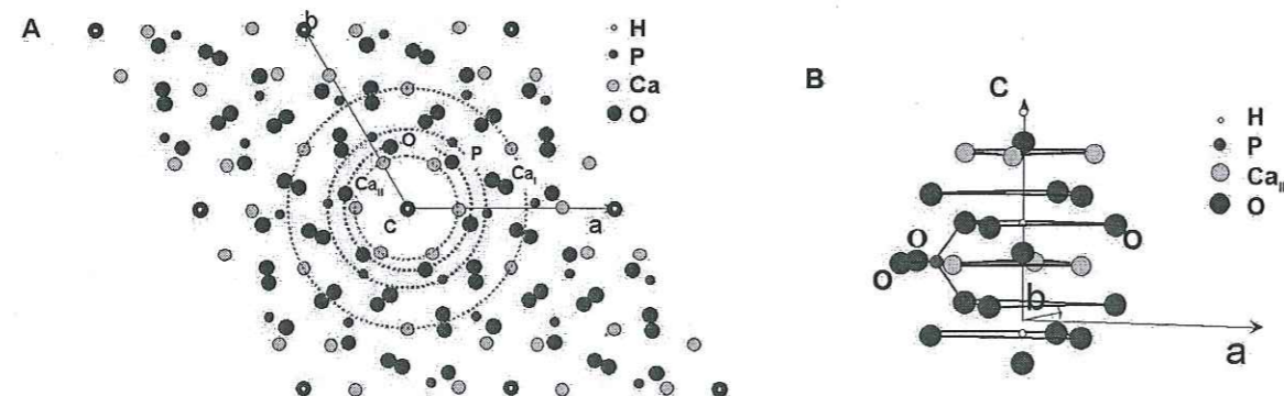
Figure 6.3: Molecular structure of hydroxyapatite viewed A) above the (001) crystallographic plane (4 unit cells are drawn, surrounding a "channel") and B) perpendicular to this plane, along the channel axis.
