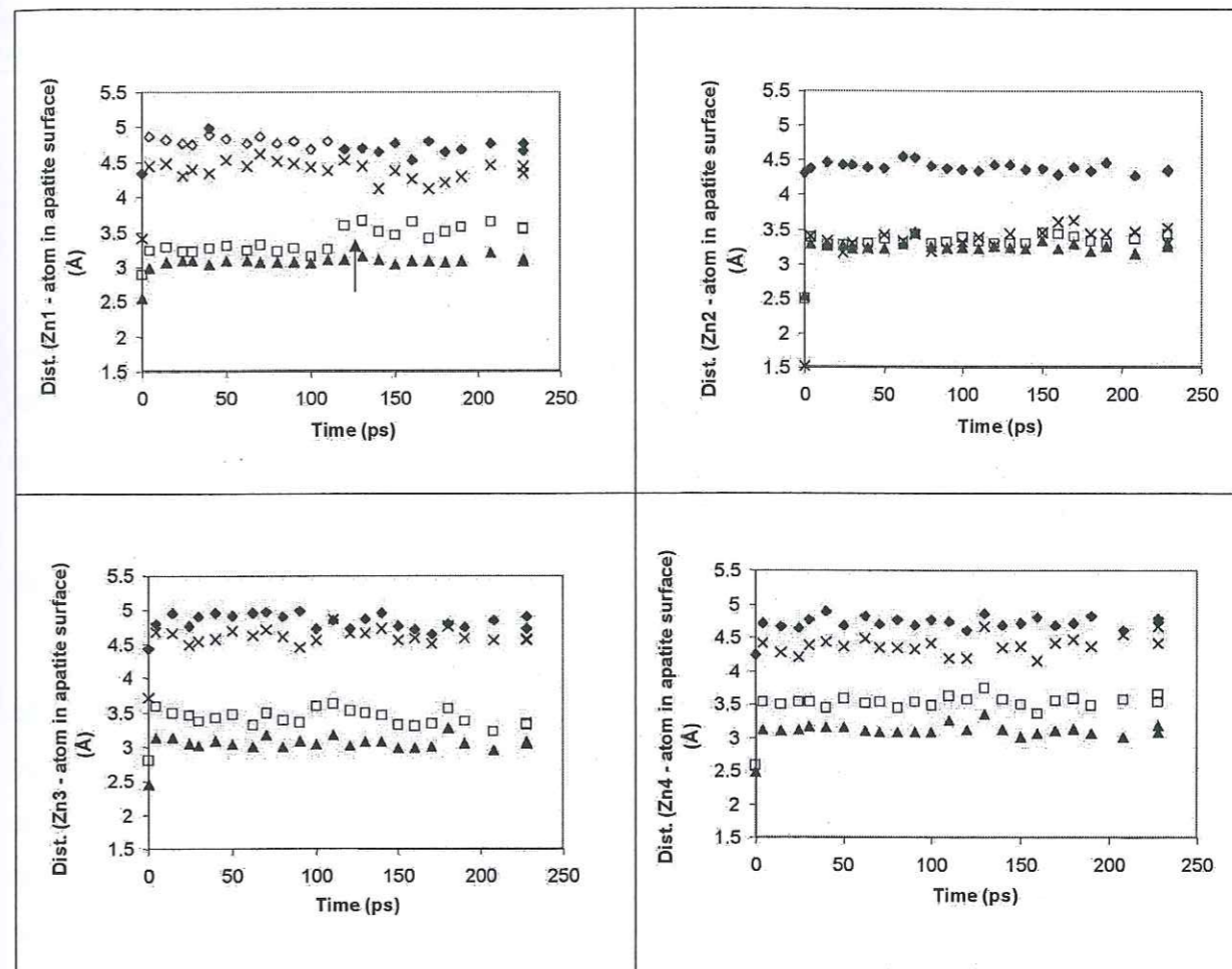
Figure 6.13: Distance between zinc ions and the surface P (triangles), CaII (squares), OH (cross) and CaI (diamonds), ) as a function of reaction time. Filled and empty diamonds correspond to 2 different CaI atoms
