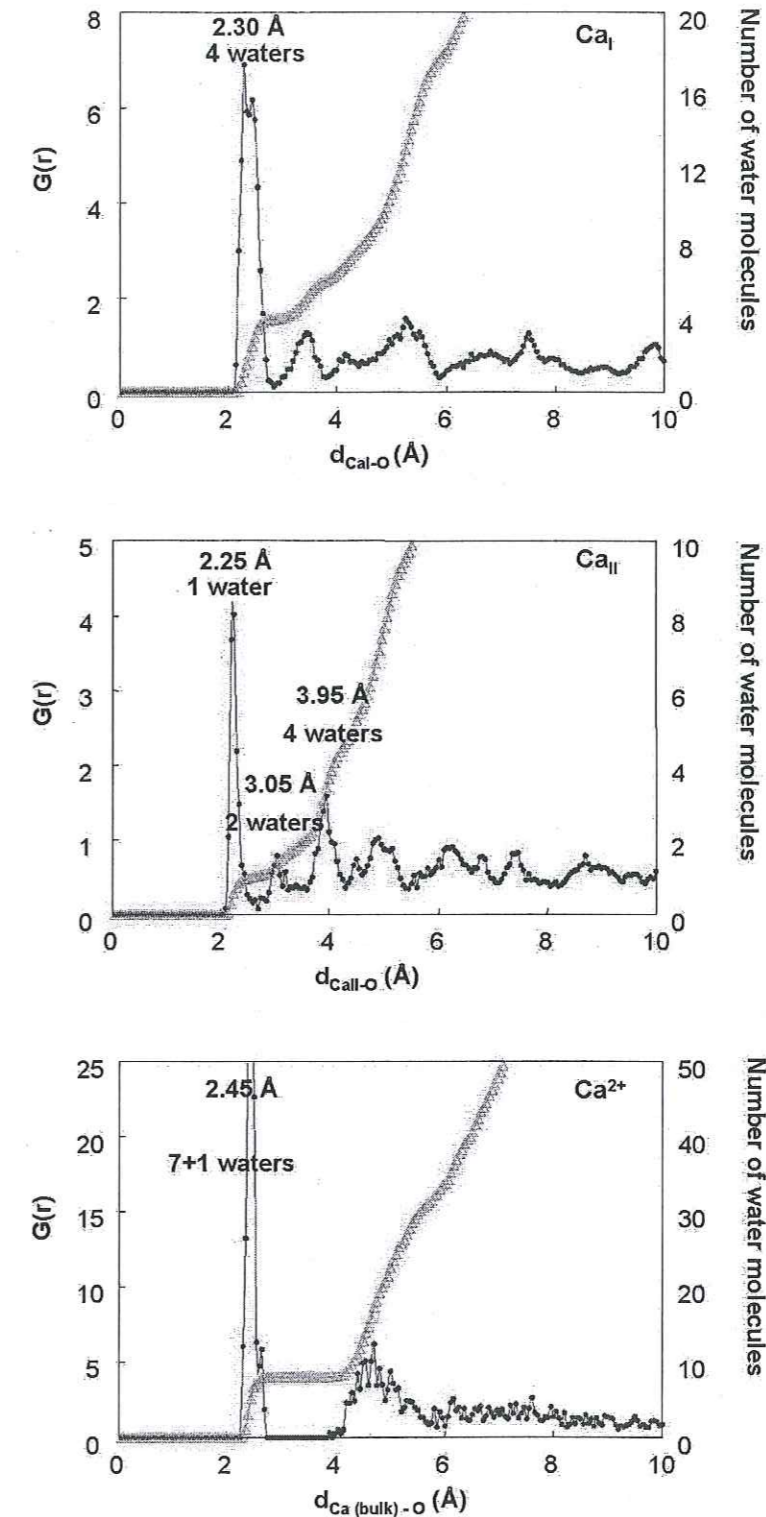
Figure 6.8 : RDF of: (a) apatite Ca_I atom at the 0-plane, (b) apatite Ca_{II} atom (around of the channel of OH) closest to the apatite surface and (c) Ca^{2+}_{(aq)} cation in water bulk. G(r) : points and number of water oxygen neighbours: triangles. Calcium atoms are surrounded by four, one and eight water molecules for apatite Ca_I atom, apatite Ca_{II} atom and water bulk Ca^{2+} cation respectively.
