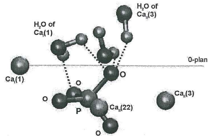
Figure 6.7: Structural environment of a phosphate ion at the apatite/water interface after 158 ps. The nearest surface Ca_I and Ca_{II} atoms and water molecules are presented. Possible hydrogen bonds are represented with dotted line.
