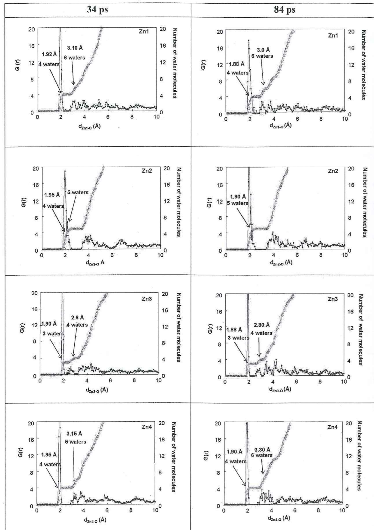
Figure 6.10 : RDF of Zinc ion at the apatite/water at different reaction times (34 ps and 84 ps). The four zinc ions at time 0 ps are positioned different distance from
