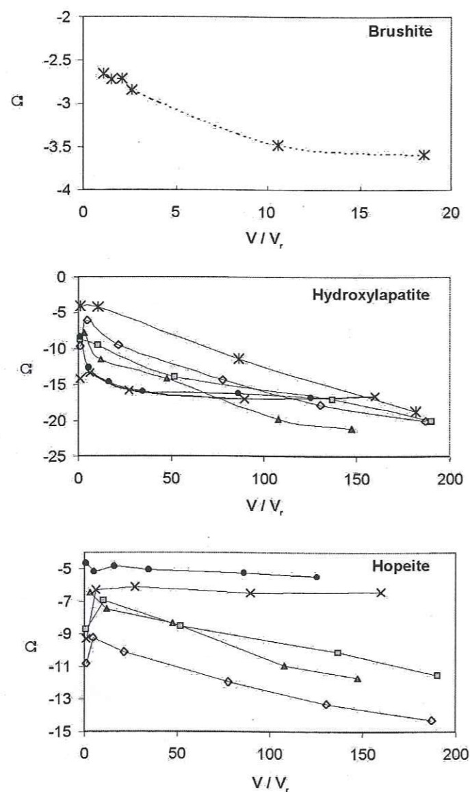
Figure 7.6: Output solution saturation index with respect to brushite (Log K = -19.03, NANCOLLAS and TOMAZIC (1974)), hydroxylapatite (Log K = -57.5, VAN CAPPELLEN (1991)) and hopeite (Log K = -32.04, VAN DER LEE (1998)). C_0 = 200 \mu\text{mol L}^{-1} (circles), 100 \mu\text{mol L}^{-1} (crosses), 13 \mu\text{mol L}^{-1} (squares), 10 \mu\text{mol L}^{-1} (triangles), 1 \mu\text{mol L}^{-1} (diamonds) and 0 (double crosses).
