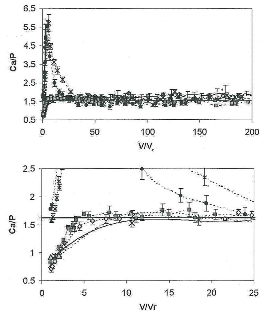
Figure 7.9: Calcium to phosphate total outflow concentration ratio C_0 = 200 \mu\text{mol L}^{-1} (circles), 100 \mu\text{mol L}^{-1} (cross), 13 \mu\text{mol L}^{-1} (squares), 10 \mu\text{mol L}^{-1} (triangles), 1 \mu\text{mol L}^{-1} (diamonds) and 0 (cross and solid line).
