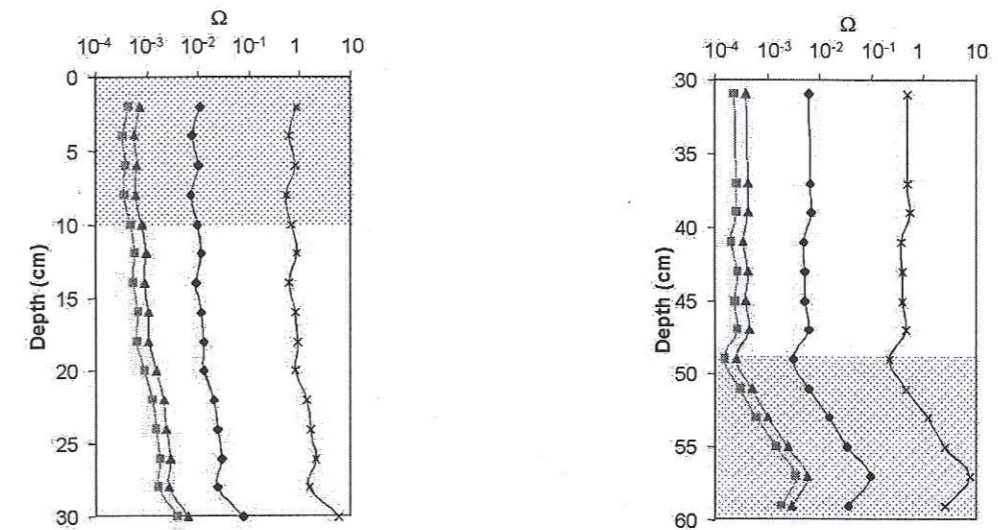
Figure 8.5: The saturation state of \text{PO}_4 in the environment A and B. \text{Ca}_5(\text{PO}_4)_3\text{OH} (crosses), \text{Ca}_3(\text{PO}_4)_2 (diamonds), \text{CaHPO}_4 (triangles), \text{CaHPO}_4 \cdot 2\text{H}_2\text{O} (squares).
