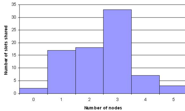
Figure 4.13: Slot reuse.
