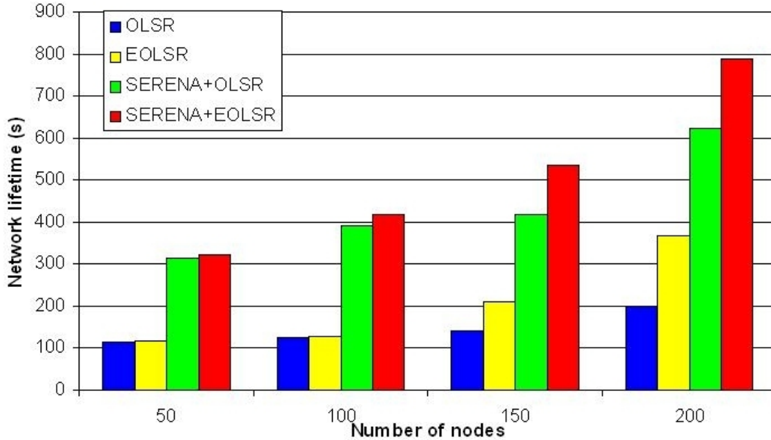
Figure 6.7: Network lifetime.
