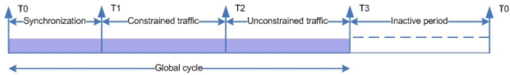
Figure 6.5: Global cycle.
