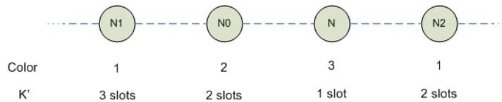
Figure 4.17: Slot assignment
