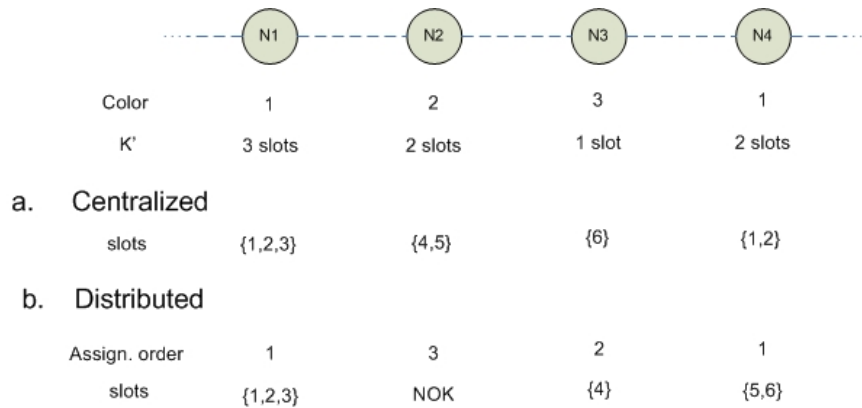
Figure 4.7: Distributed vs centralized slot assignment algorithm
