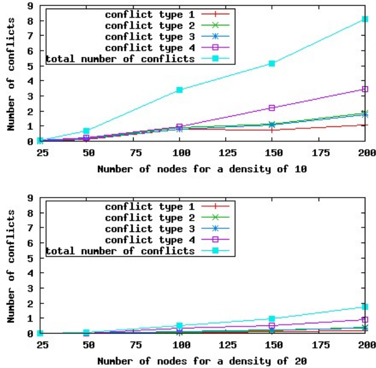
Figure 4.26: Number of conflicts per type.
