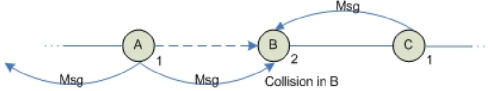
Figure 4.24: Type 3 color conflict between A and C causing a collision in B .
