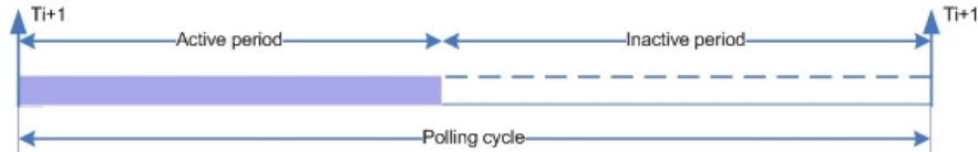
Figure 5.9: The active period in the polling cycle.
