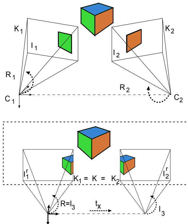
Figure 5.4: Illustration of differences between non-rectified (top) and rectified (bottom) cameras set-up. Note that the camera parameters in rectified configurations share the same \mathbf{K}, \mathbf{R} = \mathbf{I}_3 and are just shifted by a t_x translation along the x axis.
