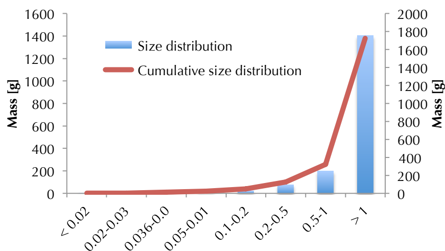
Figure 8.3 Size distribution of the KS5 debris (in [mm])
