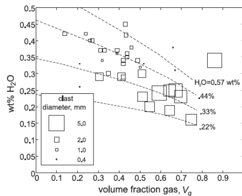
Figure 2.23 Amount of dissolved water versus gas volume fraction, squares are proportional to ash diameter [11.49]
