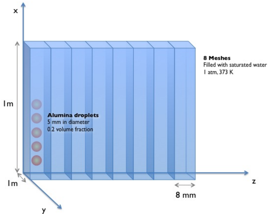
Figure 4.28 Scheme of model for MC3D calculations
