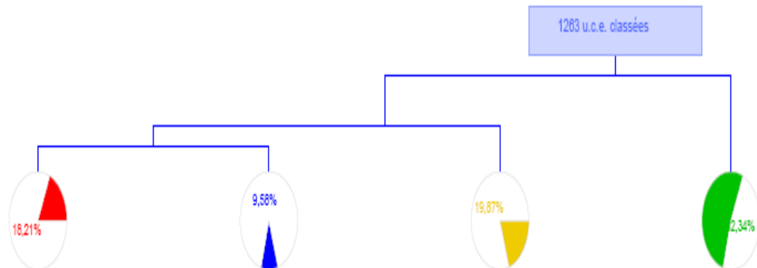
Figure 11 Dendrogramme
