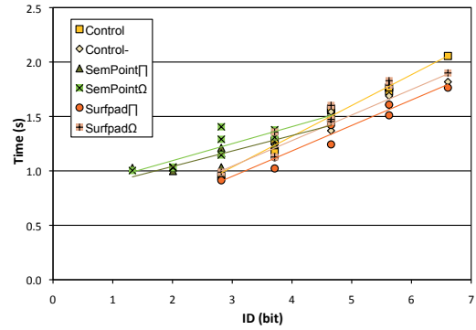
Figure 6. Fitts' law regression for each TECHNIQUE. IDs were computed in visual space for Control , Control- , SurfpadOmega and SurfpadII and motor space for SemPointII and SemPointOmega .
