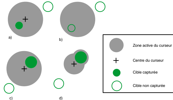
FIGURE 1.17 – Bubble Cursor
