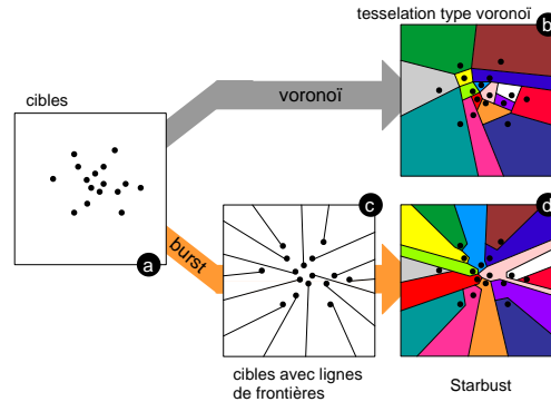
FIGURE 1.19 – Starbust
