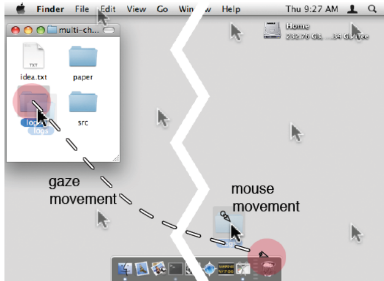
FIGURE 1.25 – Rake Cursor
