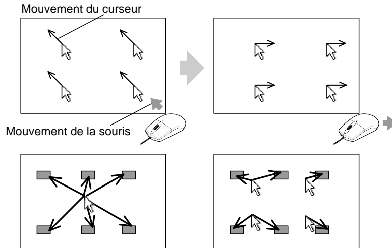
FIGURE 1.24 – Ninja cursors
