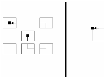
FIGURE 1.23 – Object Pointing
