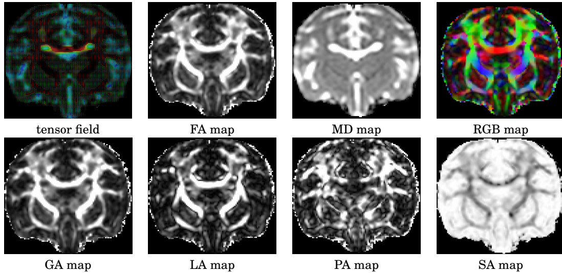
Figure 4.7: Tensor field and the scalar maps estimated from the monkey data with b = 1500s/mm^2 described in Appendix B.
