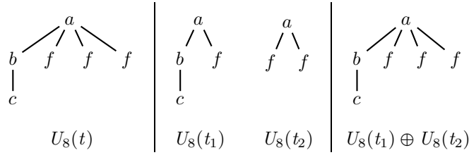
Figure 6.4: Equivalence between U_8(t) and U_8(t_1) \oplus U_8(t_2) .
