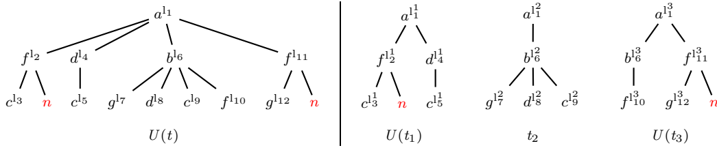
Figure 6.16: Partitioning update scenario on the input document t and its parts, for a given iterative update U .
