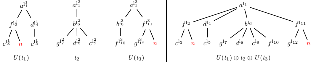
Figure 6.17: Fusion scenario on distinct (updated and non-updated) parts.
