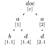
(2) The projector \pi_1 for u_1
