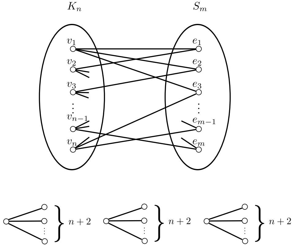
Figure 4.1: The graph H of the reduction in Theorem 4.2.1
