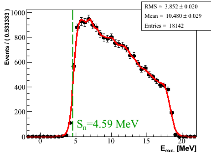
Figure 4.6: Simulated excitation energy spectrum of the detected protons from deuteron break-up. The spectrum starts slightly before the neutron separation energy due to the detector resolutions.
