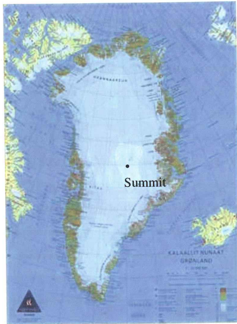
Fig. 7: Map of Greenland with the ice core-drilling site of Summit.
