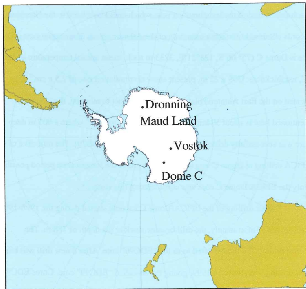
Fig. 6: Map of Antarctica with the drilling sites illustrated in sections 4.1.1 and 4.1.2.
