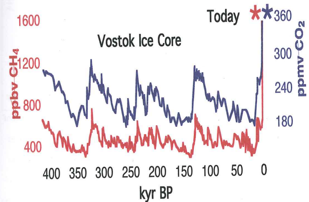
Fig. 3: Greenhouse gases ( CH_4 and CO_2 ) variations in the Vostok Antarctic ice core during the last 420 kyr [Petit et al. , 1999]. These parameters are co-varying with T and evidence that climate has changed with a strong 100 kyr cycle during the late Quaternary, alternating long glacial ages with short interglacial periods.
