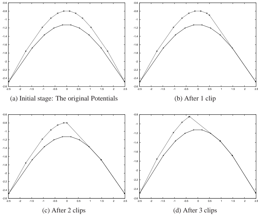
Figure 3.1: Counter clockwise clipping of the potential: the first 3 steps
