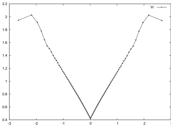
Figure 3.2: Conditional variance: clipping tails first
