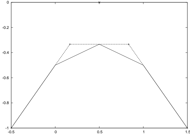
Figure 2.1: The potentials of the two measures before L2 quantization
