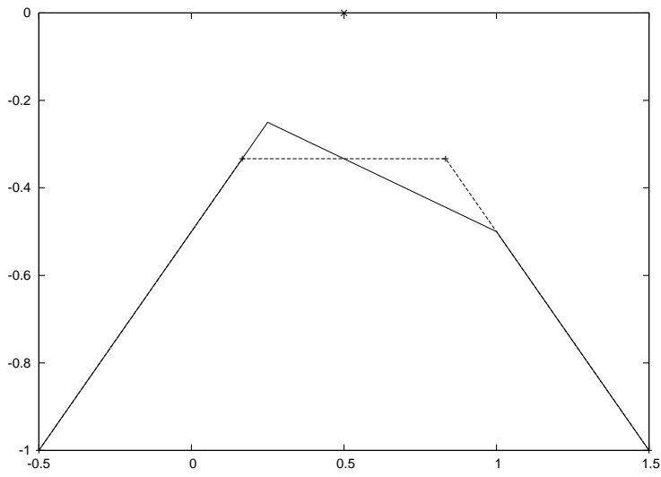
Figure 2.2: The potentials of the two measures after L2 quantization (note that by Criterion 1 of section 2, neither of the quantized measures dominates the other in the convex order).
