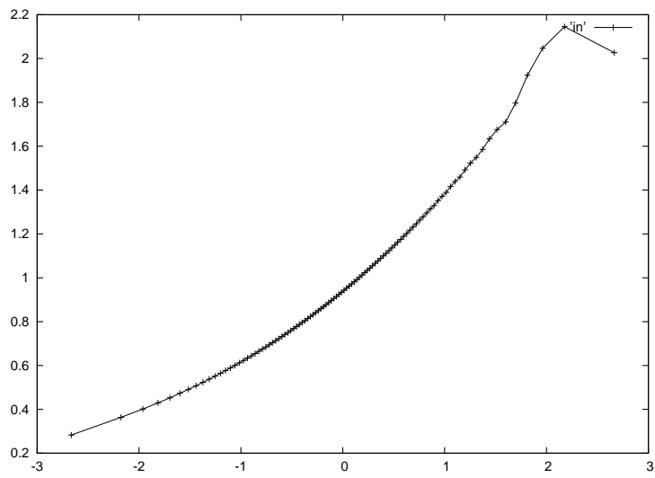
Figure 3.4: Conditional variance: clipping counterclockwise
