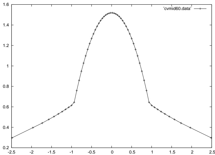
Figure 3.3: Conditional variance: clipping from center to extremities
