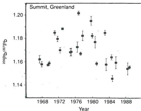
FIG. 1 Changes in the 206 Pb/ 207 Pb ratio in Greenland snow between 1967 and 1988. The uncertainties given are 95% confidence intervals. The crescent-shaped trend is mainly due to combined changes in both the isotopic composition and the consumption of leaded gasoline in the United States.
