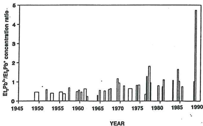
Figure 4. Concentration ratio \text{Et}_2\text{Pb}^{2+}/\text{Et}_3\text{Pb}^+ found in a snow core from the Summit site.
