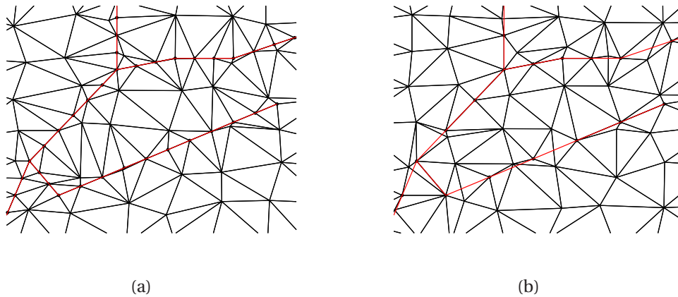
Figure 4.18: Close-up of the mesh resulting from a crack discretisation of (a) 3 \times 10^{-4} m and (b) 7 \times 10^{-4} m
