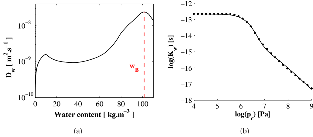
Figure 4.12: (a) Moisture diffusivity and (b) permeability profiles, including Durner model interpolation
