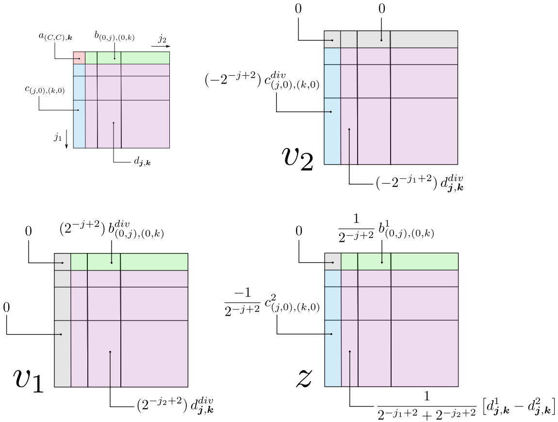
Figure A.2: Multiscale divergence-free decomposition/reconstruction schemes. Top left: disposition of coefficient sets a (red), b (green), c (blue), d (pink). v_1 coeff. from z coeff. (Eq. (A.15), bottom left ); v_2 coeff. from z coeff. (Eq. (A.16), top right ); z coeff. from v_1, v_2 coeff. (Eq. (A.17), bottom right ).
