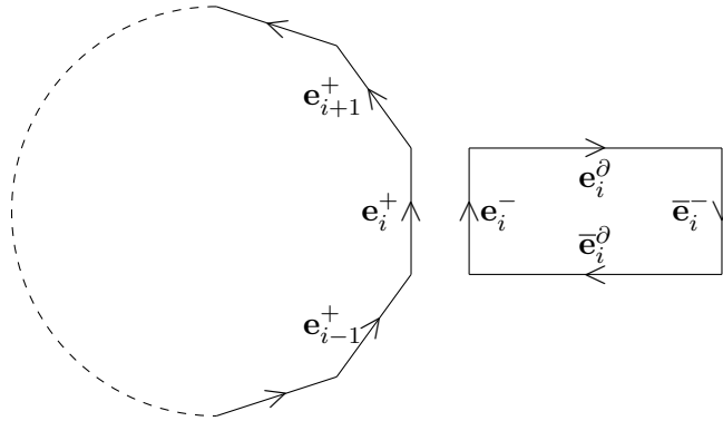
Figure 4.2: Construction of the thickened graph S(\Gamma) .
