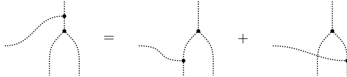
Figure 1.7: The IHX relation.
