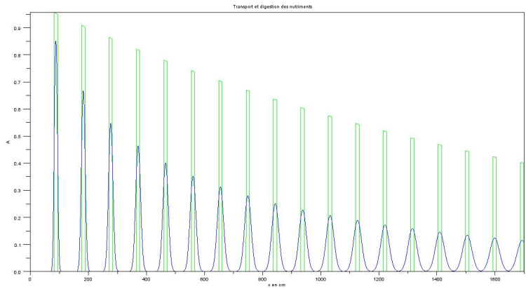
(b) \Delta x = 0.25\text{cm}, \Delta t = 1\text{s}
