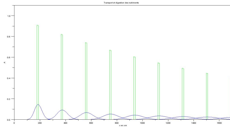
(a) \Delta x = 5\text{cm}, \Delta t = 4\text{s}
