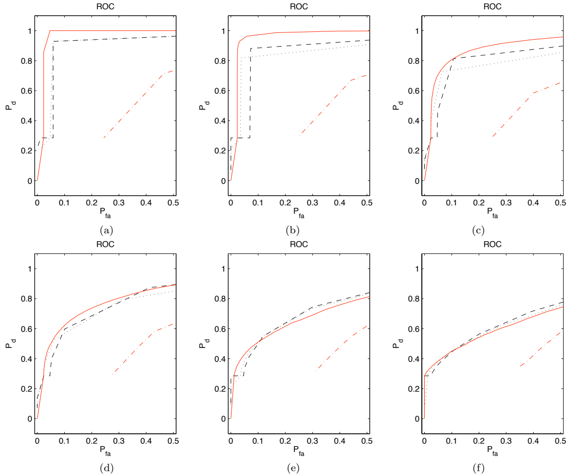
Figure 4.5: ROCs computed for synthetic test signal in Figure 4.4(a) using E^{(1)} (dotted line), E^{(w)} (dashed line), TDH^{(w)} (continuous line), and wavelet + higher order statistics (dash-dotted line). N_{points} = 100 points are computed on each ROC curve, which is the average of N_{rep} = 500 repetitions. (a) \text{SNR} \rightarrow \infty ; W = 6 ; E^{(2)} ; TDH^{(4)} . (b) \text{SNR} = 15 dB; W = 5 ; E^{(4)} ; TDH^{(4)} . (c) \text{SNR} = 10 dB; W = 4 ; E^{(3)} ; TDH^{(4)} . (d) \text{SNR} = 7 dB; W = 4 ; E^{(3)} ; TDH^{(4)} . (e) \text{SNR} = 5 dB; W = 5 ; E^{(2)} ; TDH^{(3)} . (f) \text{SNR} = 3 dB; W = 3 ; E^{(2)} ; TDH^{(2)} .
