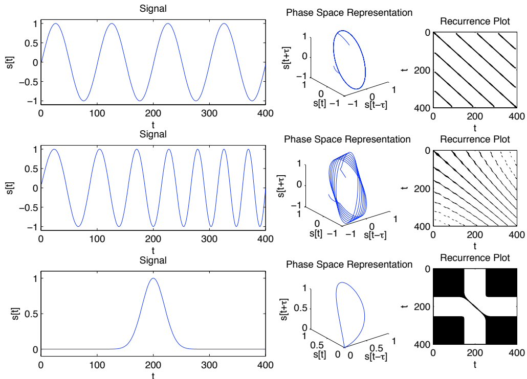
Figure 3.4: Examples of typical signals and their corresponding recurrence plots. (top) Sinusoidal signal. (middle) Chirp signal. (bottom) Gaussian pulse.
