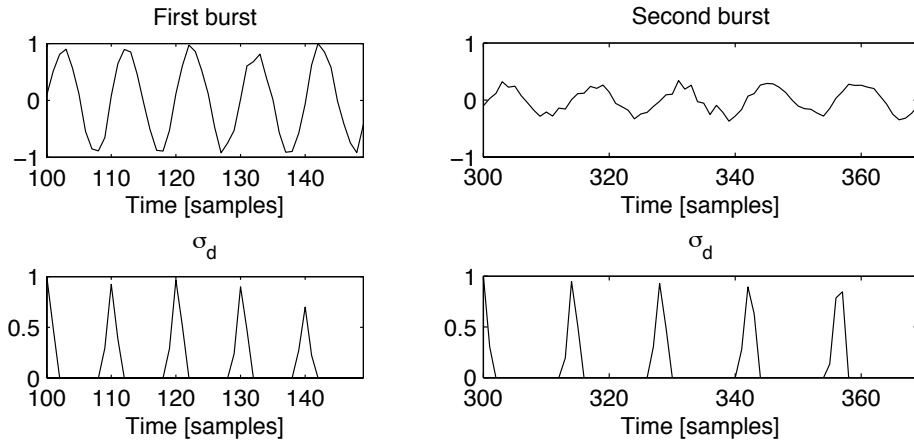
Figure 4.17: The RQA measure \sigma_d , computed for the two transients in the test signal in Figure 4.12, using w = 7 and \varepsilon = \varepsilon_0 .
