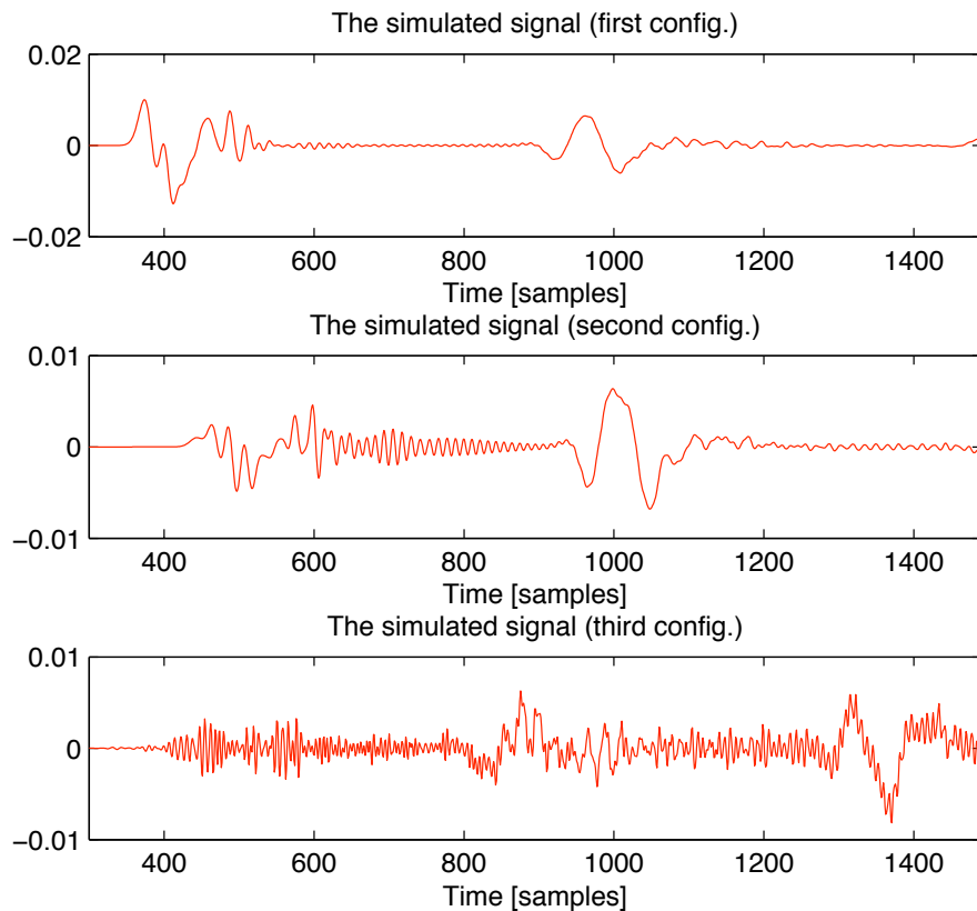
Figure 5.16: The received signals obtained for the angle beam transducer experiment. (The real signals were shown in Figure 5.7.)
