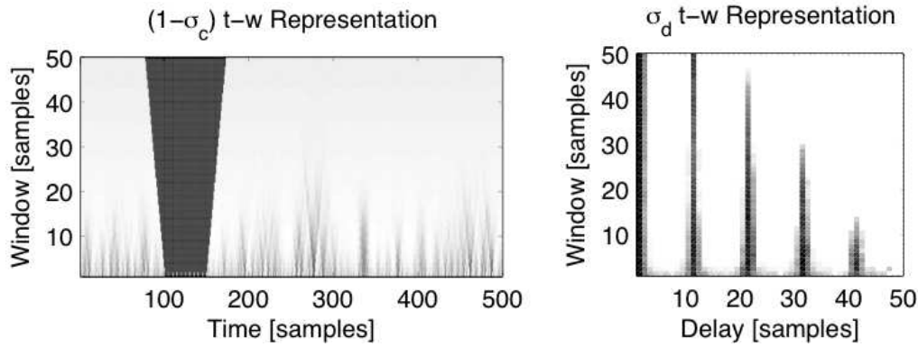
Figure 4.3: The \bar{\sigma}_c^{(\varepsilon)} and \sigma_d^{(\varepsilon)} t - w representations, computed using \varepsilon = \varepsilon_0 .
