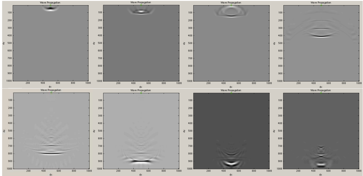
Figure 5.11: Snapshots of wave propagation for the simulation of the first experiment. (The time advances from left to right, and from top to bottom.)
