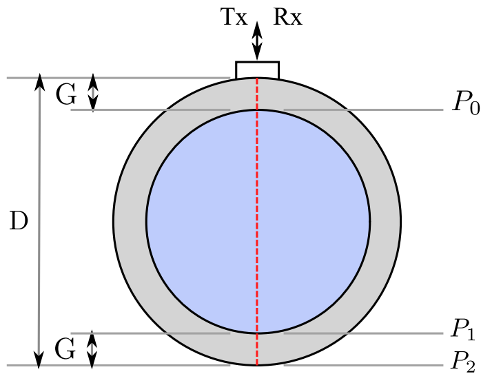
Figure 5.5: The the pipe section, for the straight beam transducer experiment.
