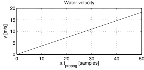
Figure 5.26: The values of the water velocity, v , with respect to the propagation time difference, \Delta t_{\text{propag}} .
