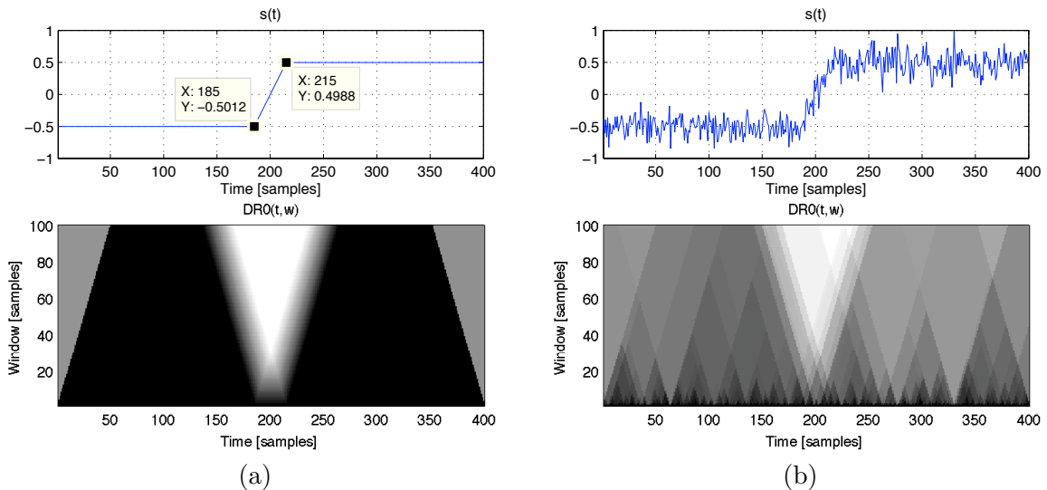
Figure 3.13: A signal containing two stable states and a linear transition between them, and the dynamic range norm computed for each of its vector samples, in a t - w representation. The length of the plateau is minimal for values of w around 30, i.e. the duration of the ramp. (a) No noise case. (b) SNR = 10 dB case.
