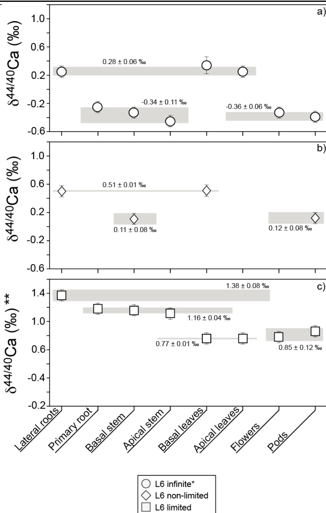
Figure IV.3 : \delta^{44/40}\text{Ca} composition in various bean organs in the plant for (a) L6 infinite, (b) L6 non-limited and (c) L6 limited experimental conditions. * from Cobert et al. (2011a). ** values corrected for the bias related to the use of the two Ca salts used in the experiment.
