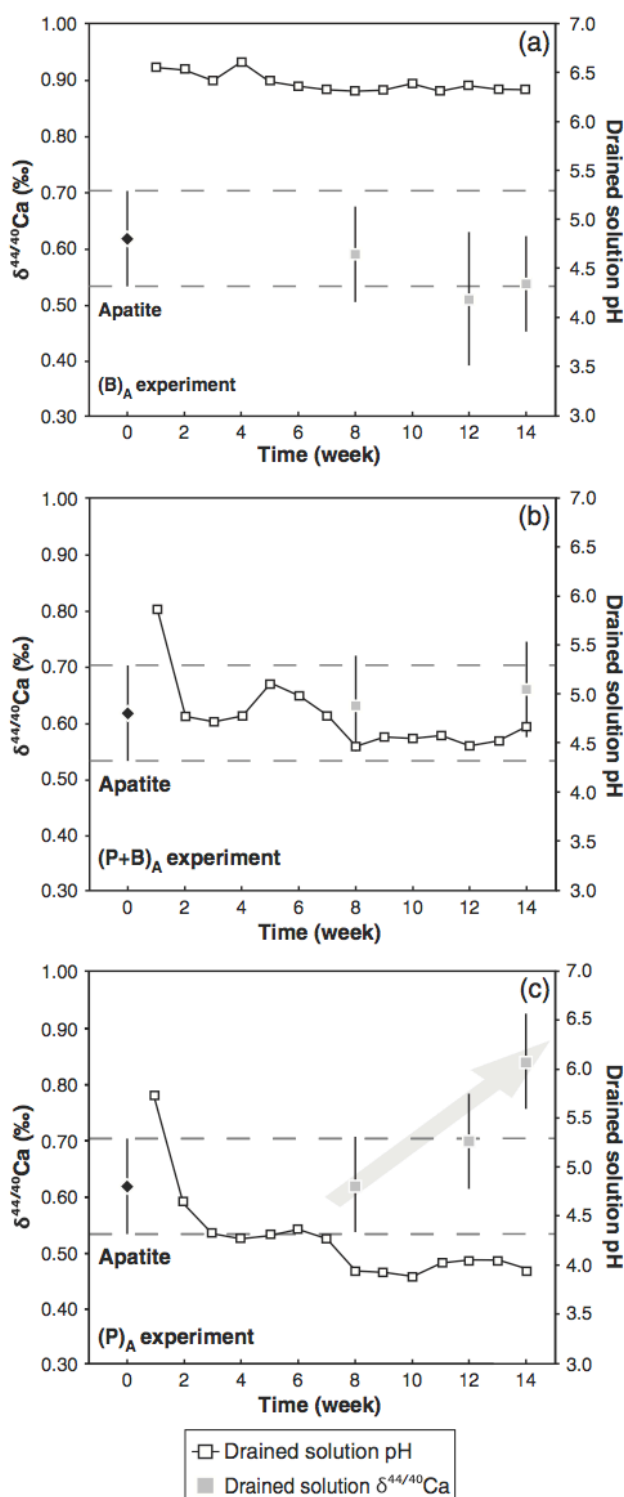
Figure 2. Evolution of Ca isotopic compositions and pH values of the collected percolates through time for columns filled with apatite and (a) B. glathei PML1(12) bacteria ((B) A ); (b) B. glathei PML1(12) inoculated Scots pine ((P+B) A ); and (c) not inoculated Scots pine ((P) A ).
