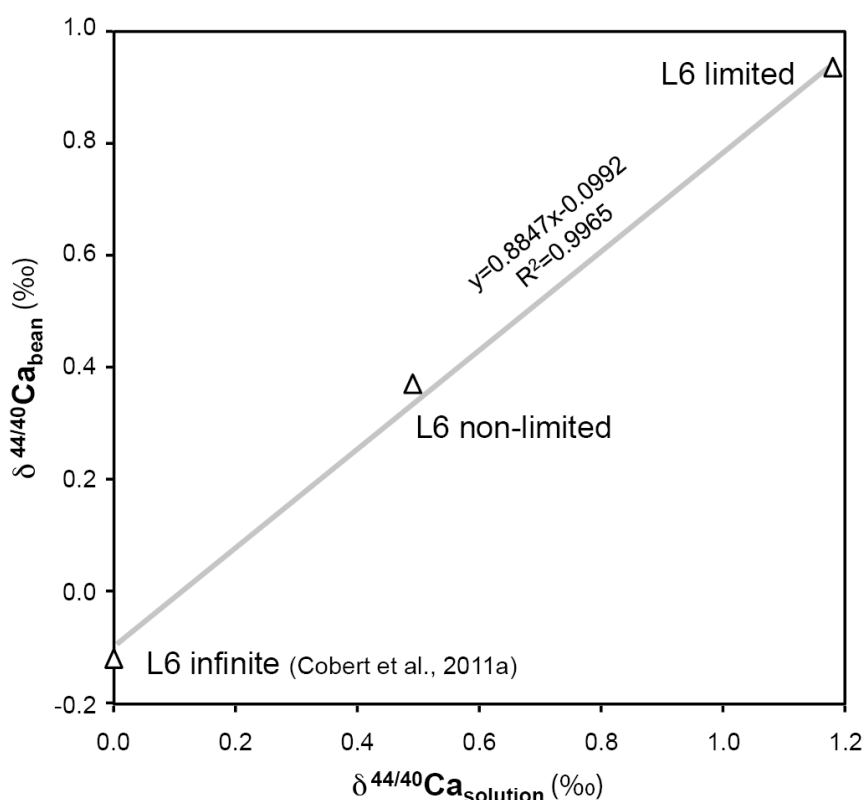
Figure IV.5 : \delta^{44/40}\text{Ca}_{\text{bean}} versus \delta^{44/40}\text{Ca}_{\text{solution}} relationships for the 3 experimental L6 conditions (infinite, non-limited and limited).
