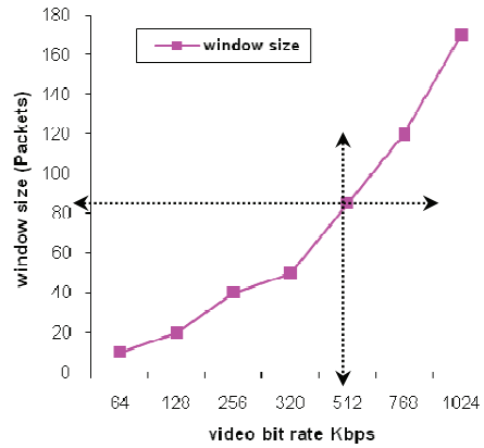
Figure 7. 18: Window size for different video rates against video rates (64K, 128K, 256K, 512K, 768K and 1M)
