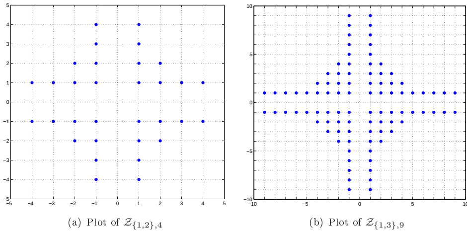
FIGURE 5.2 – Illustration of crosses \mathcal{Z}_{\mathbf{u}, \beta_{\mathbf{u}}} .
