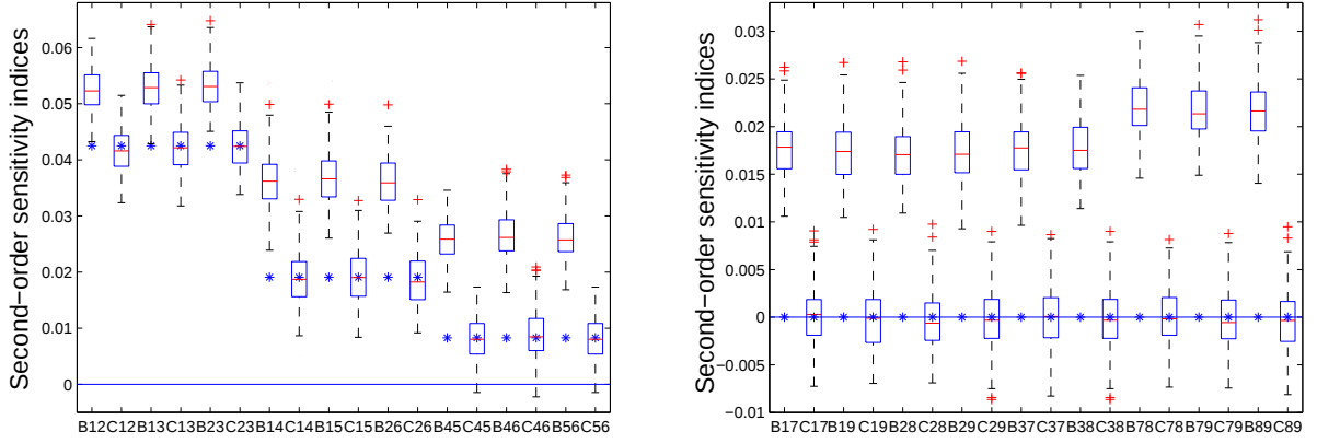
FIGURE 4.4 – Estimation of the second-order SI using RBD-FAST. We compare, for a fixed sample size N = 4001 , the basic estimator (Bij) with the bias-corrected one (Cij). In each column, we mark the theoretical SI with a blue asterisk and plot several summaries of a sample of 200 estimator replicates : the red central mark is the median ; the box has its lower and upper edges at the 25 th percentile q and the 75 th percentile Q , respectively ; the whiskers extend between q - 1.5(Q - q) and Q + 1.5(Q - q) ; the red crosses are outliers.
