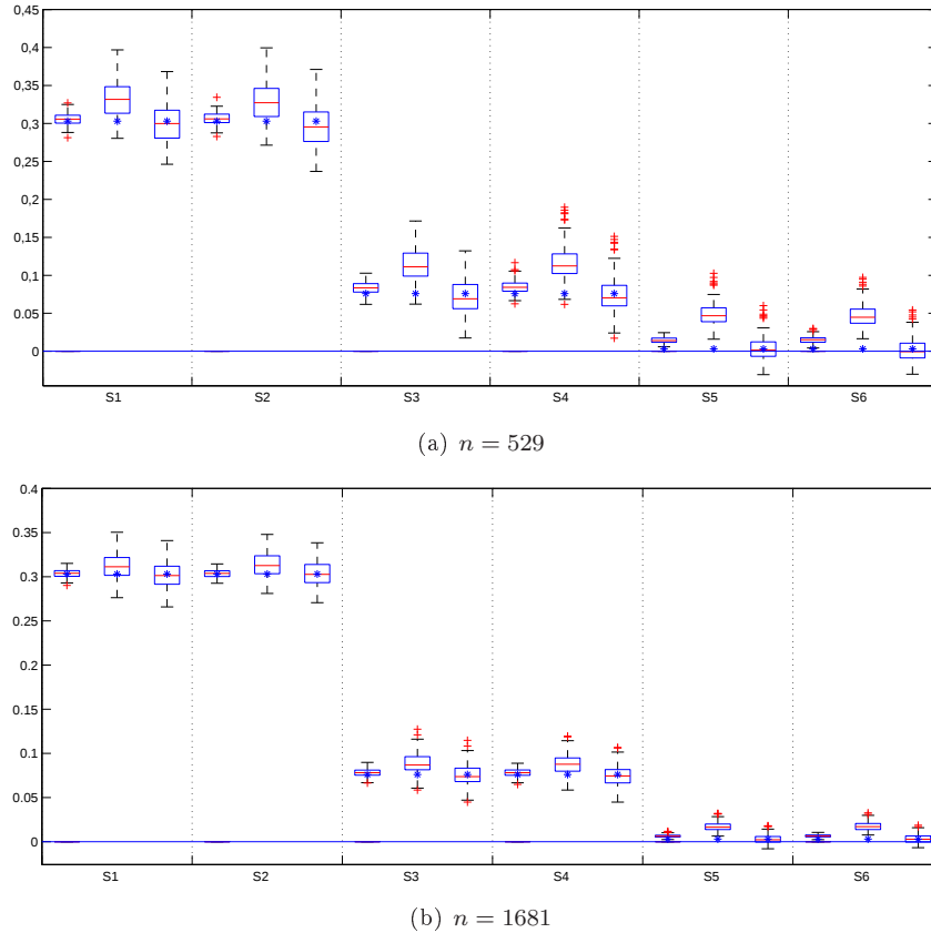
FIGURE 5.3 – Boxplots of the first-order sensitivity indices estimates. For each sensitivity index, S_1, S_2, \dots, S_6 , from the left to the right are \hat{S}_i(\mathcal{R}_1 f, \mathcal{Z}_{\{i\}, 12}, A_2(\boldsymbol{\pi})) (strength 2 orthogonal array, without bias correction), \hat{S}_i(\mathcal{R}_1 f, \mathcal{Z}_{\{i\}, 12}, A_1(\boldsymbol{\pi})) (strength 1 orthogonal array, without bias correction), \hat{S}_i^c(\mathcal{R}_1 f, \mathcal{Z}_{\{i\}, 12}, A_1(\boldsymbol{\pi})) (strength 1 orthogonal array, with bias correction), respectively.
