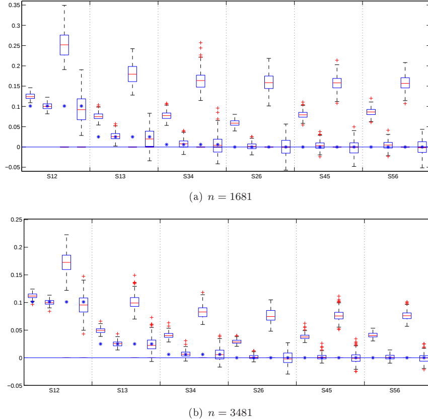
FIGURE 5.4 – Boxplots of the second-order sensitivity indices estimates. For each sensitivity index, S_{12} , S_{13} , \dots , S_{56} , from the left to the right are \hat{S}_{ij}(\mathcal{R}_1 f, \mathcal{Z}_{\{i,j\},12}, A_{2,n}(\boldsymbol{\pi})) (strength 2 orthogonal array, without bias correction), \hat{S}_{ij}^c(\mathcal{R}_1 f, \mathcal{Z}_{\{i,j\},12}, A_{2,n}(\boldsymbol{\pi})) (strength 2 orthogonal array, with bias correction), \hat{S}_{ij}(\mathcal{R}_1 f, \mathcal{Z}_{\{i,j\},12}, A_{1,n}(\boldsymbol{\pi})) (strength 1 orthogonal array, without bias correction), \hat{S}_{ij}^c(\mathcal{R}_1 f, \mathcal{Z}_{\{i,j\},12}, A_{1,n}(\boldsymbol{\pi})) (strength 1 orthogonal array, with bias correction), respectively.
