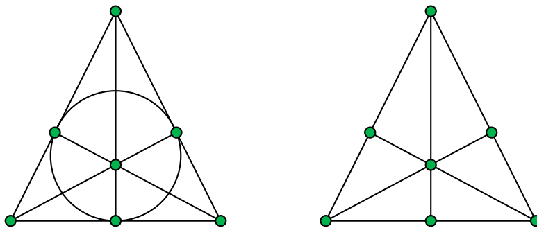
Figure 3.6: The Fano and the non-Fano matroids
