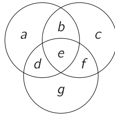
Figure 2.10: Representation of the region for three random variables
