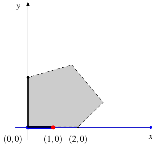
Figure 6.5: Geometric intuition for an essentially conditional inequality which is not valid for almost entropic points
