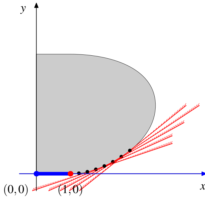
Figure 6.4: Geometric intuition for an essentially conditional inequality for almost entropic points
