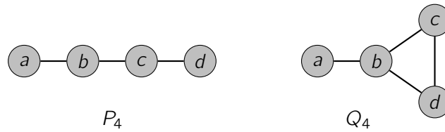
Figure 3.5: P_4 and Q_4 : the excluded induced subgraphs for complete multipartite graphs
