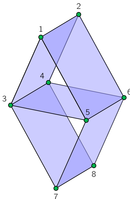
Figure 3.8: A picture of the Vámos matroid
