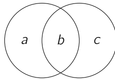
Figure 2.9: Representation of the region for two random variables
