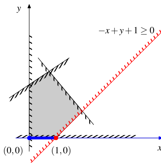
Figure 6.3: Geometric intuition for a trivial conditional inequality
