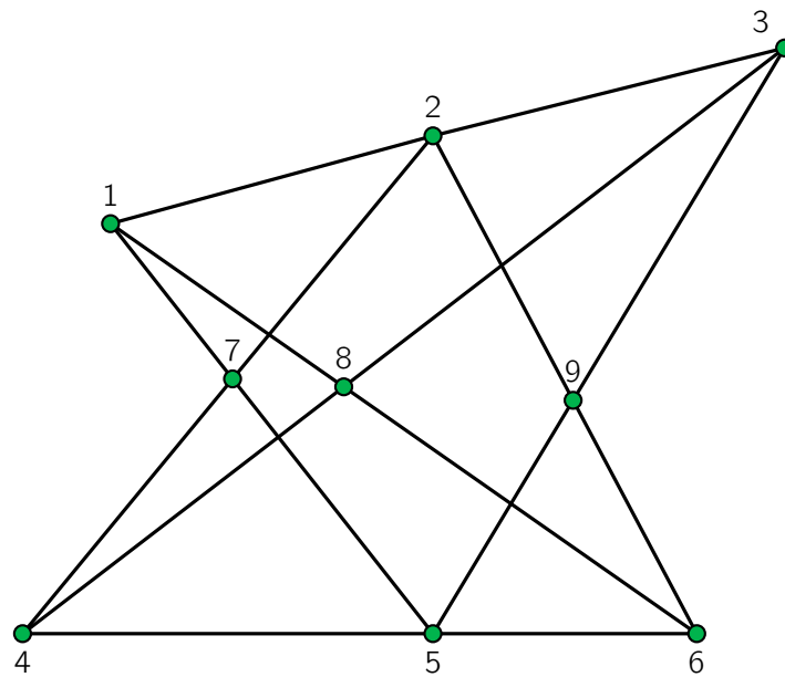
Figure 3.7: A picture of the non-Pappus matroid
