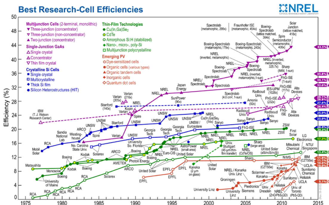
Figure 1.2. Efficiency evolution of best research cells by technology type. This table identifies those cells that have been measured under standard conditions and confirmed at one of the world's accepted centres for standard solar-cell measurements. Source: NREL, 2012.
