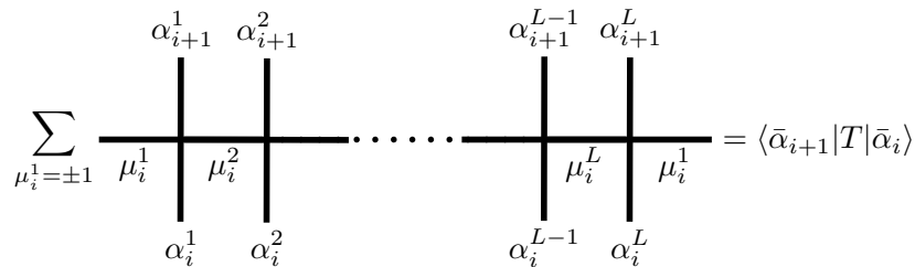
Figure IV.7: Graphical representation of the transfer matrix of the six-vertex model.
