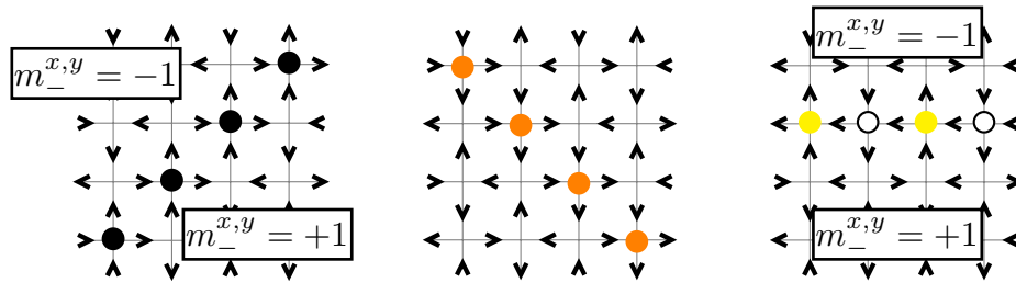
Figure VI.18: Domain walls between AF domains of opposite staggered order. The configuration of arrows is shown. We use the colour rule defined in Fig. VI.2. Left panel: diagonal walls in the \parallel direction are made of a -vertices. Central panel: diagonal walls in the \perp direction are made of b -vertices. Right panel: horizontal (and vertical, by symmetry) walls are made of an alternating chain of a - and b -vertices.
