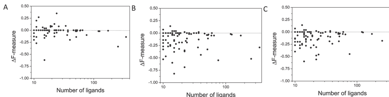
Figure 5: Difference in the F-measure value ( \Delta F -measure) of three chemogenomic models (KTL1, KTL2, KTL3) in classifying 2 882 true target-ligand PDB complexes and 11 528 target-ligand decoys: (A) F(KTL1)-F(KTL2) , (B) F(KTL1)-F(KTL3) , (C) F(KTL2)-F(KTL3) . Values are plotted according to the number of true ligands for each binding site cluster.
