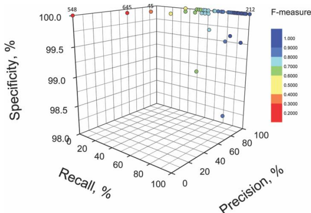
Figure 3: Recall, specificity, and precision of 87 SVM local models using the KTL3 target-ligand kernel. Data are color-coded according to the F-measure value. Binding site clusters discussed in the text are labeled according to their number.
