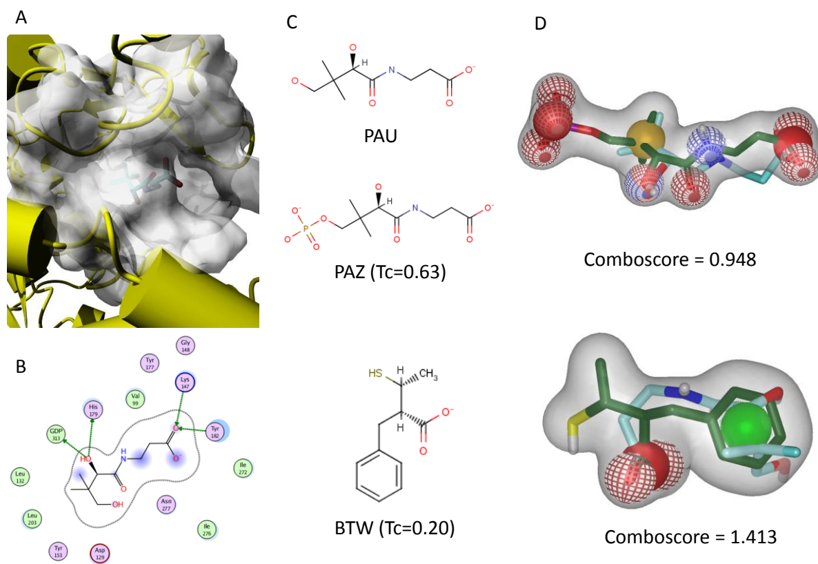
Figure 6: Profiling pantothenic acid (HET code = PAU). (A) X-ray structure of PAU (sticks) in complex with pantothenate kinase (white surface, pdb entry 3af0). (B) Schematic 2-D diagram of protein-ligand interactions. Apolar and polar binding site residues are circled in green and violet, respectively. Hydrogen-bonds are indicated by green arrows. Accessible ligand atoms are enclosed by a cyan dot. (C) Chemical structures of PAU, PAZ, and BTW ligands. 2-D similarity to PAU is indicated in brackets. (D) ROCS overlay of PAU (cyan carbon atoms) with PAZ and BTW (green carbon atoms). Oxygen, nitrogen, and sulfur atoms are colored in red, blue, and yellow, respectively. The shape of templates (PAZ, BTW) is displayed by a white surface. Pharmacophoric features are displayed by balls (H-bond acceptor, red mesh dot; H-bond donor, blue meshed dot; negative ionizable, red solid dot, hydrophobe, yellow dot; and ring, green dot).
