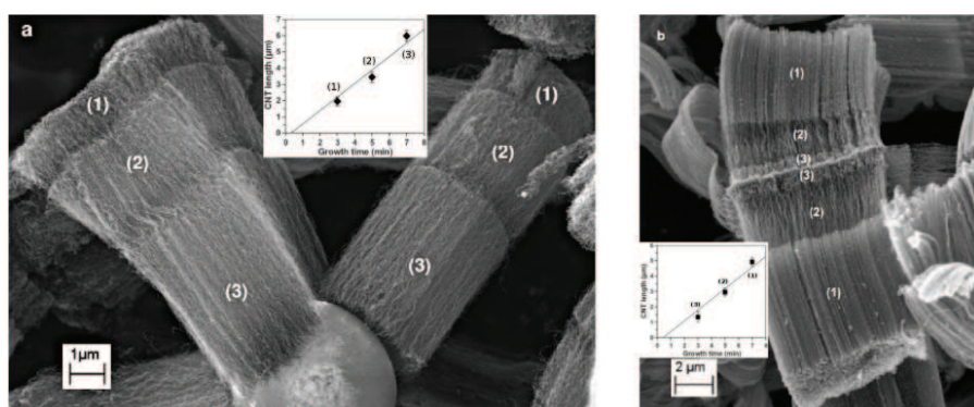
Figure 6.1.1: SEM images showing a 3 stack of aligned CNT layers on \mu\text{-Al}_2\text{O}_3 (a) and on \mu\text{-SiC} (b). Three separated growth sequences with the same conditions but different growth time were used [31].
