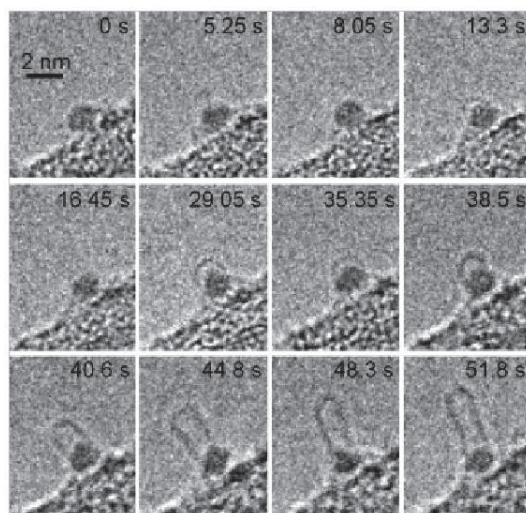
Figure 1.5.7: Atomic scale in situ observations of catalyst during CNT growth by CVD [99].
