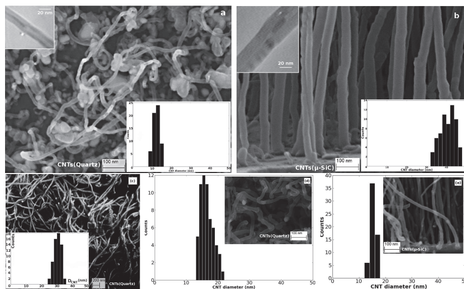
Figure 3.3.1: Electron microscopy images and diameter distribution of the resulting CNTs grown under the smaller (a) and the larger (b) conditions. The images presented in (c), (d) and (e) correspond to CNTs grown under the Taguchi conditions 1, 2 and 5, respectively.
