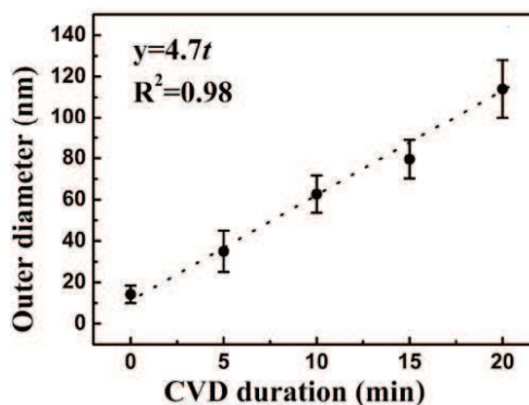
Figure 6.4.2: Variation of the CNT diameter with the deposition time. The error bars correspond to the diameter distribution.
