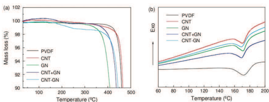
Figure 1.3.3: The (a) TGA and (b) DSC curves of PVDF and its different composites with 6.6 wt% fillers (CNT-GN hybrid, CNT+GN mixture, GNs and CNTs) [32].
