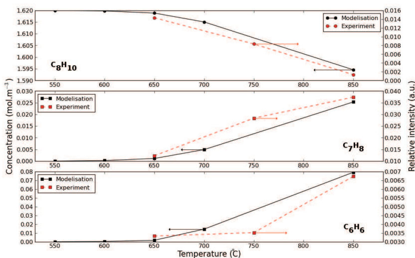
Figure 4.2.2: Comparisons between experimental (red dotted lines) and theoretical (black straight lines) concentration evolutions of C_8H_{10} , C_7H_8 and C_6H_6 at the middle of the CVD reactor as a function of the temperature.
