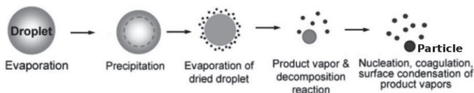
Figure 4.4.2: Schematic of the nanoparticle formation in floating CVD based on [129].
