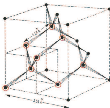
Figure 1.1.4: Schematic of the diamond structure.
