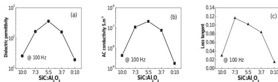
Figure 5.2.5: Dependence of the dielectric permittivity (a), the AC conductivity (b) and the loss tangent (c) of the PVDF and CNT-based hybrids composites with different \text{SiC}/\text{Al}_2\text{O}_3 mass ratio.
