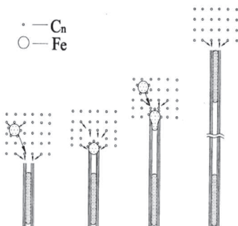
Figure 1.5.3: A proposed continuous CNT growth model based on an opened tip-growth mechanism [186].
