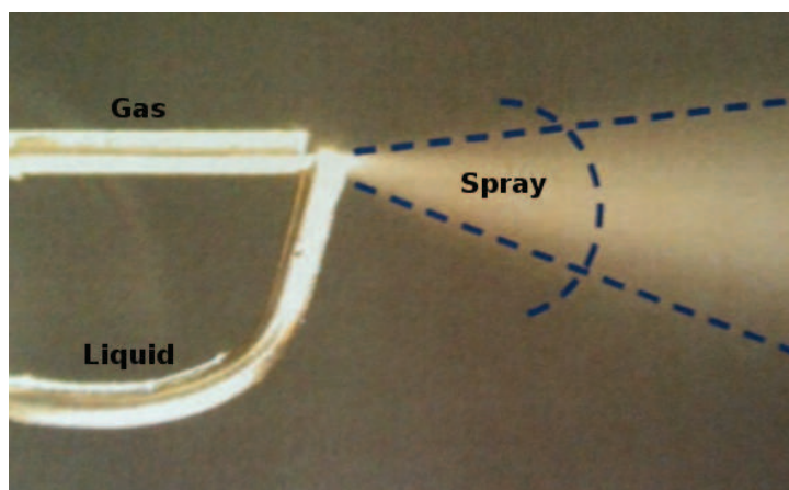
Figure 2.1.1: Image of the injection system used to spray the precursors into the CVD reactor.
