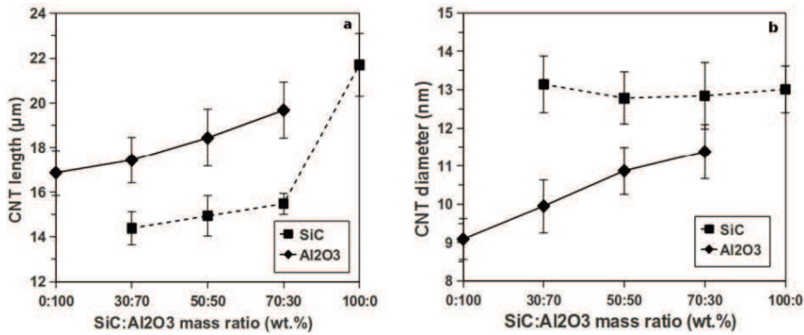
Figure 5.2.2: Evolution of the CNT length (a) and diameter (b) on both ceramic \mu -particles as a function of the SiC/Al 2 O 3 mass ratio.
