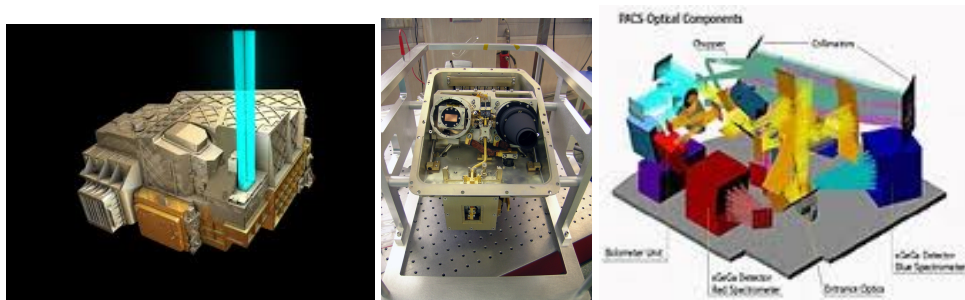
FIGURE 3.4 – L'instrument PACS.
