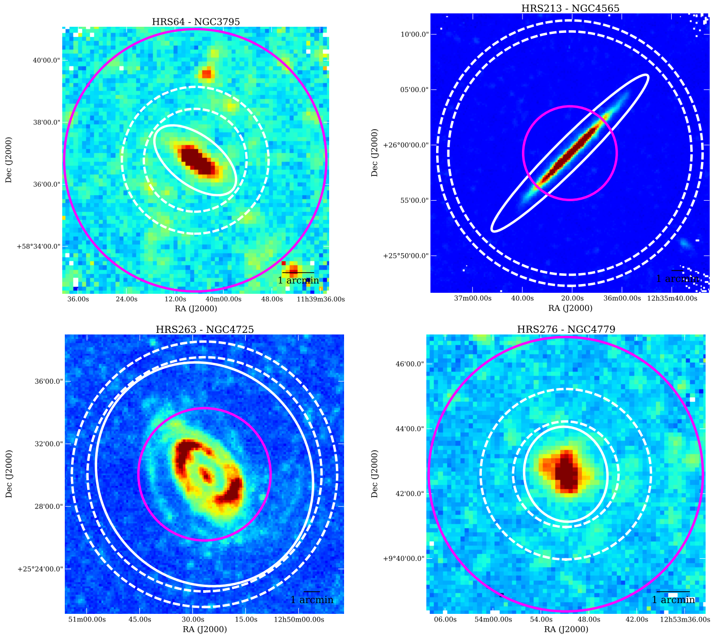
Fig. 9: Comparison between Planck and Herschel aperture photometry on 350 \mu\text{m} SPIRE images, with in white, the apertures used for Herschel photometry and in dashed white for the background estimation, in magenta the aperture used by the Planck consortium on Planck images.
