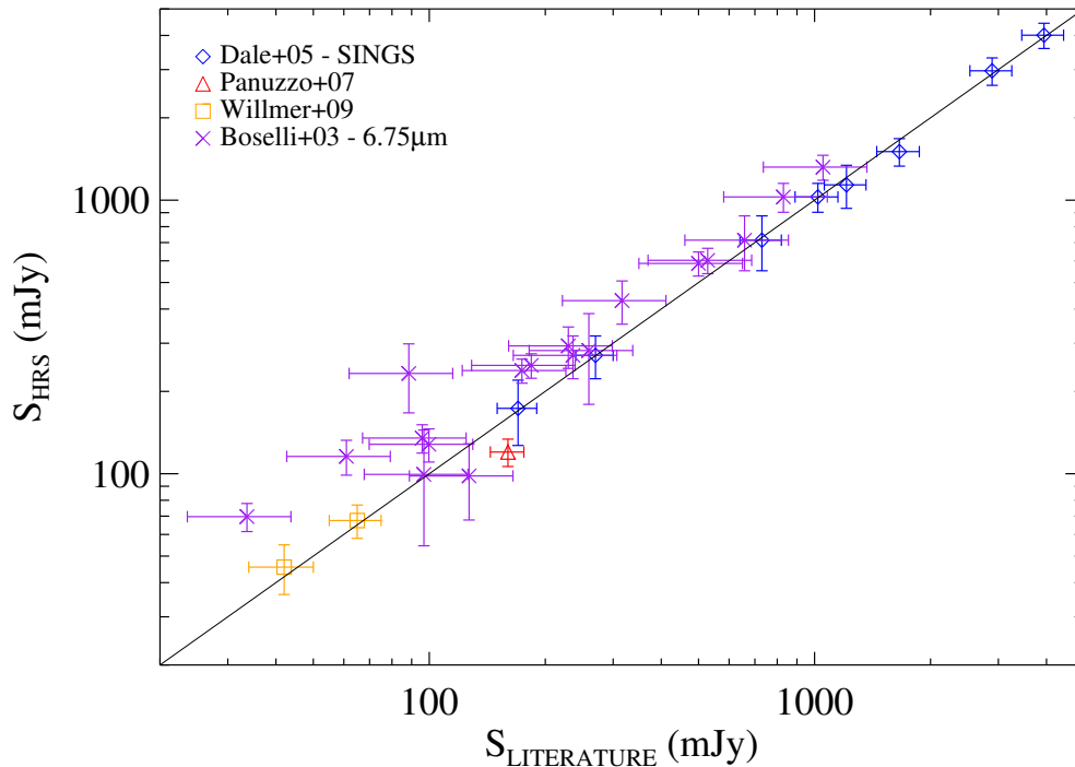
FIGURE 7.3 – Comparison between our Spitzer /IRAC flux density measurements and Spitzer /IRAC, ISO ( 6.75 \mu\text{m} ) data available from the literature for galaxies in common.
