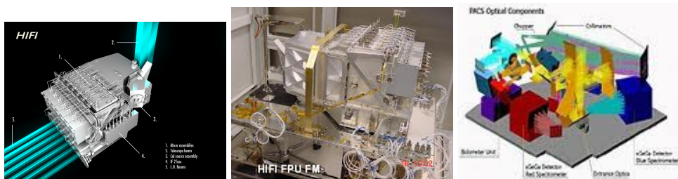
FIGURE 3.3 – L'instrument PACS.
