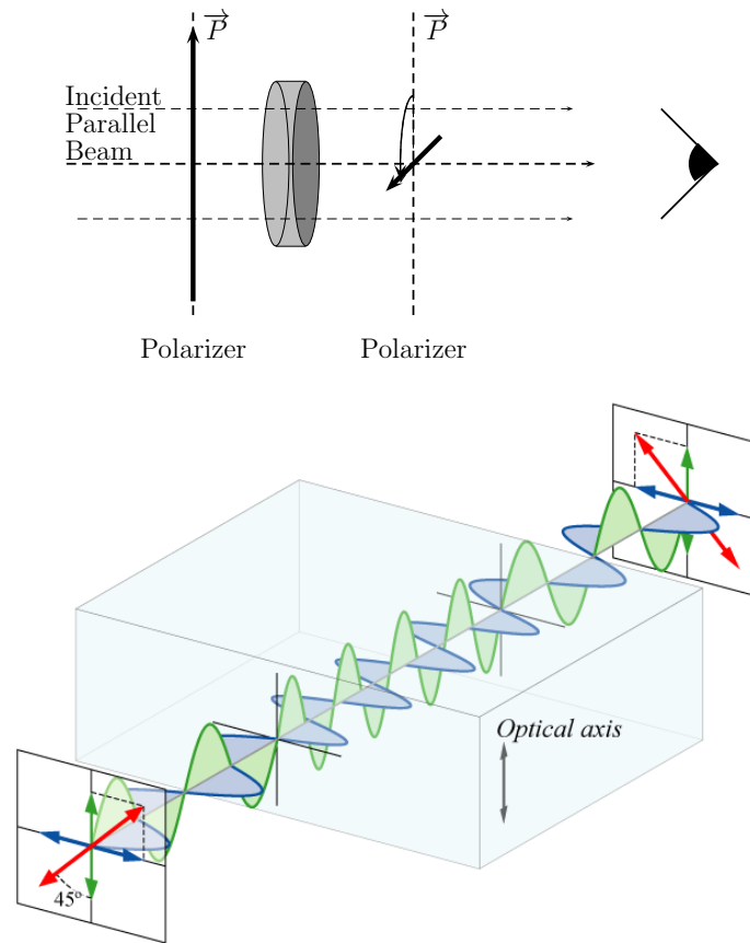
Figure 2.7: Top : Scheme of measuring birefringence setup. The material lighted by transmission between two crossed polarizers. Bottom : Fate of a polarized light (red) through a quarter wave plate with optical axes along vertical and horizontal axis. The vertical axis has a higher refraction index and the light along the vertical axis is faster. From Wikipedia.
