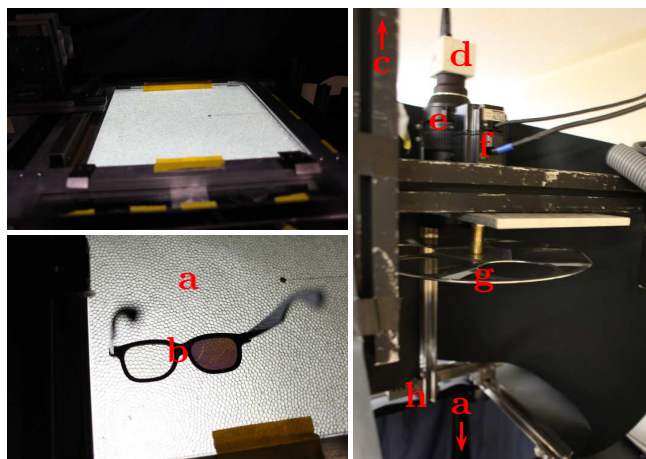
Figure 2.11: Pictures of the polarized setup. (a): photo-elastic grains lighted by transmission by a polarized backlight. (b): cheap version of the polariscope: 3D movie theater glasses. (c): ceiling. (d): camera. (e): lens. (f): stepper. (g): polariscope. (h): shelf.
