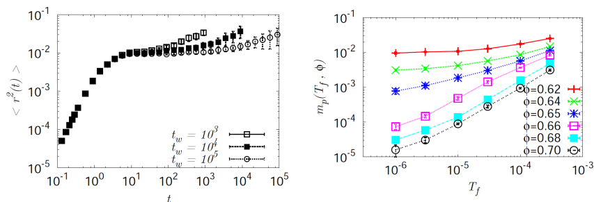
Figure 3.32: Left : Quench dependence. Mean square displacements vs. lag time at density \phi = 0.7 for different preparation protocols for harmonic spheres in 3 dimensions at finite temperature. Larger t_w is equivalent to slower preparation protocol. Right : Plateau value value of the plateau of the Mean square displacements vs. temperature for different densities. Extracted from Otsuki and Hayakawa [2011].
