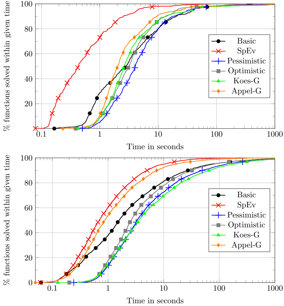
Figure 3.12: Percentage of functions that can be solved optimally in the given amount of time for EEMBC (top) and SPEC (bottom). The markers on the curves help to identify the related configuration, they do not represent the actual measurements, which would have been too dense.
