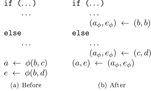
Figure 3.7: Replacement of \phi -functions.
