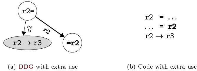
Figure 8.4: Care has to be taken that dependencies between a definition and its uses are not lost.
