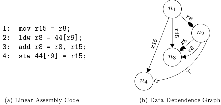
Figure 8.1: Assembly code (a) and the corresponding data dependence graph (b).
