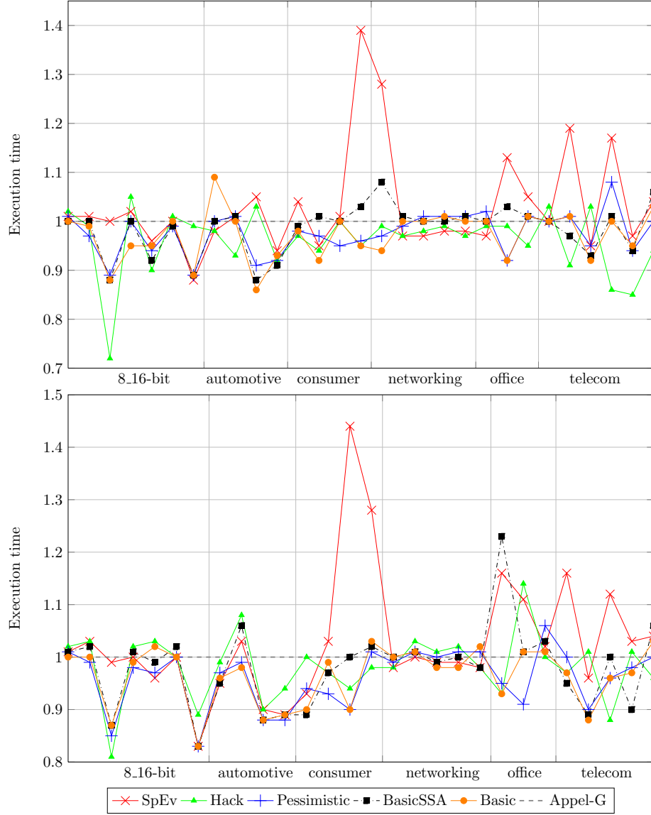
Figure 3.18: Runtime results per bench for EEMBC using frequency estimate (top) and profiling feedback (bottom). In both cases, latency optimization is performed after spilling and before coloring. (Lower is better)
