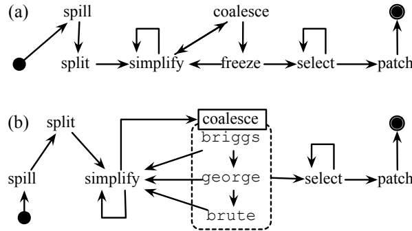
Figure 6.4: (a) A decoupled re-implementation of IRC . (b) A decoupled re-implementation of Bouchez’s BF that handles aliasing.
