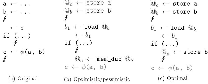
Figure 3.8: Optimal memory duplication placement.
