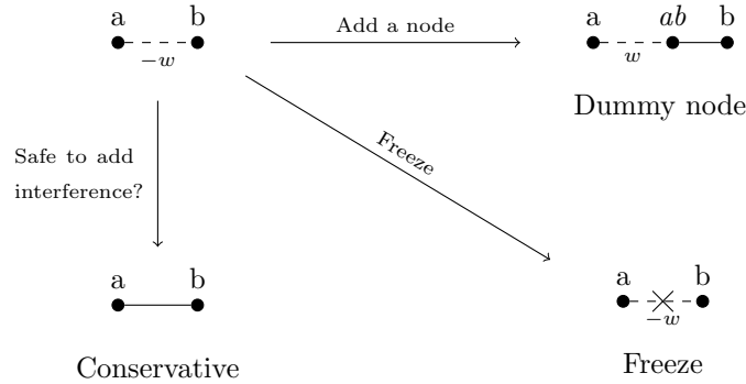
Figure 5.3: Strategies to deal with antipathies.
