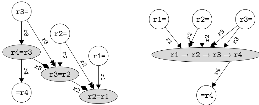
(a) DDG with a set of copy nodes
