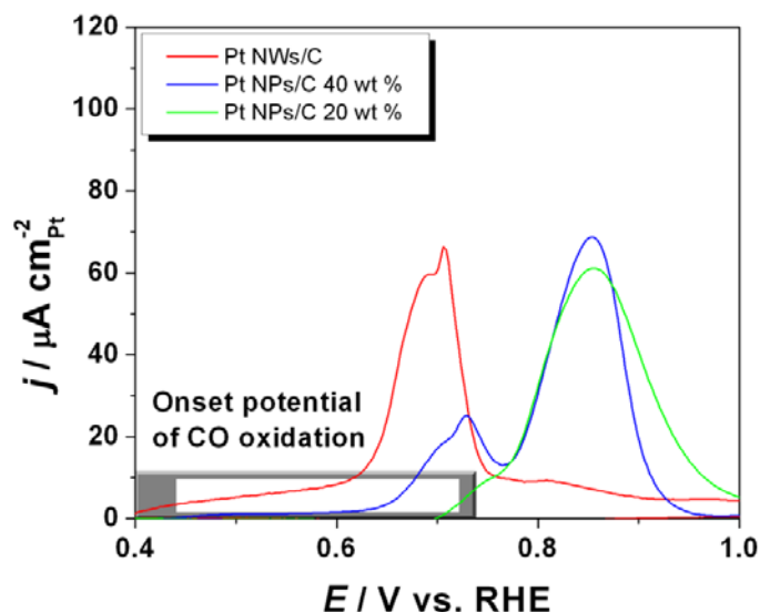
Figure VI-9. Background-subtracted CO stripping voltammograms on Pt NWs /C, Pt NPs/C 20 wt.% Pt NPs/C 40 wt.%. in 0.1 M \text{HClO}_4 , sweep rate 0.02 \text{ V s}^{-1} . Electrolyte: 0.1 M \text{HClO}_4 ; \nu = 0.020 \text{ V s}^{-1} ; T = 20 \text{ }^\circ\text{C} .
