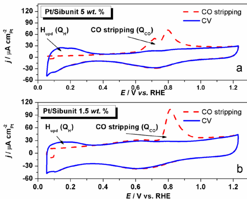
Figure V-3. The first and the second CO stripping voltammograms recorded on a Pt/Sibunit 5 wt. % (a) or on a Pt/Sibunit 1.5 wt. % (b) in CO-free 0.1 M HClO 4 . \nu = 0.020 V s -1 ; T = 20 °C.
