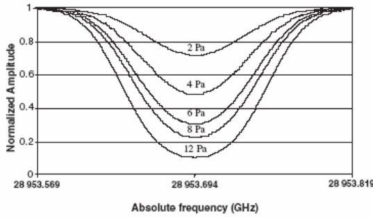
FIG. 2. Series of absorption spectra at different pressures.
