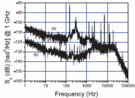
Fig. 4. Phase noise spectral density of the optical compensation system at 1 GHz in closed loop (a) with the 86-km optical fibre (b) with optical attenuators equivalent to the fibre attenuation.
