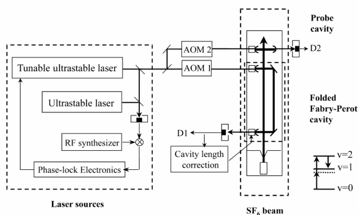
Figure 4. Experimental set-up for the Doppler-free two-photon experiment on a supersonic beam of \text{SF}_6 . (AOM: acousto-optic modulator) The molecular beam interacts with the two standing waves generated by a first Fabry–Perot cavity and in resonance with the two-photon transition between the vibrational levels v=0 and v=2 . A probe laser beam detects the population in the v=2 level.
