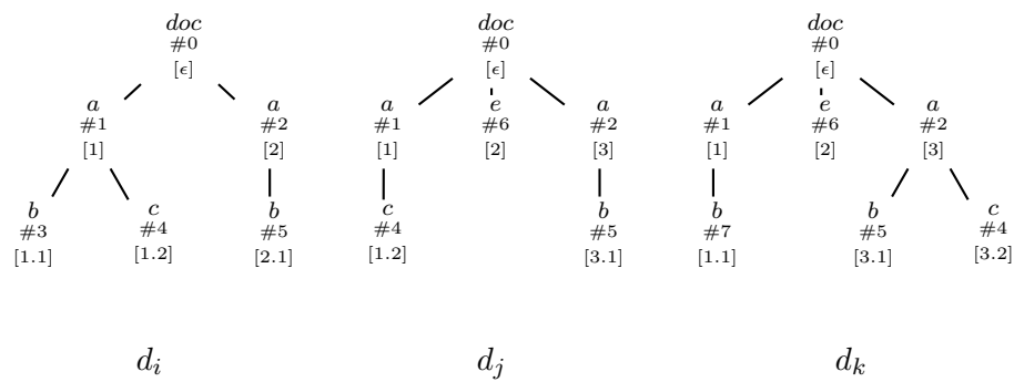
FIGURE 6.1 – Illustration des identifiants explicites.
