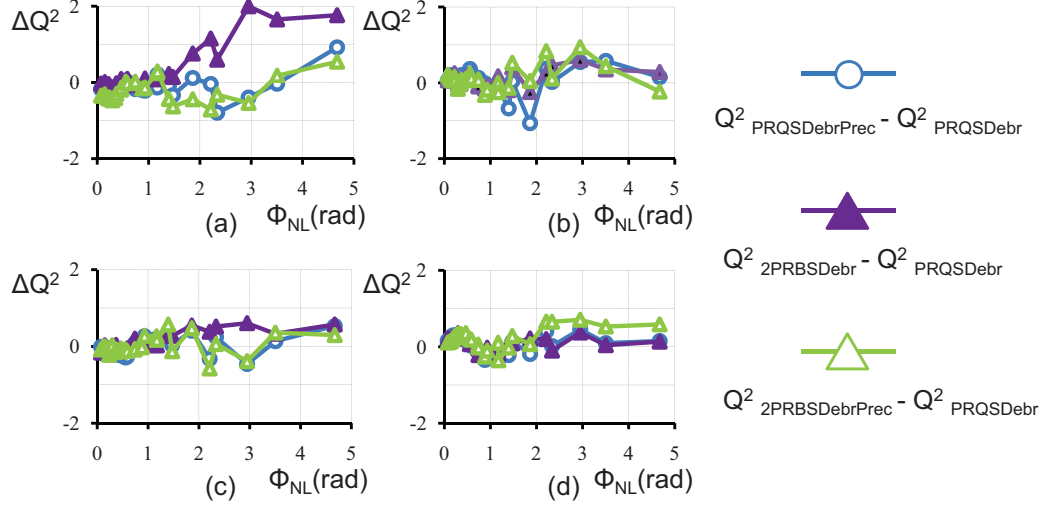
Figure 3.15: Configuration with D_{lin} = 0 \text{ ps} \cdot \text{nm}^{-1} \cdot \text{km}^{-1} (a) L_{seq} = 256 , (b) L_{seq} = 1024 , (c) L_{seq} = 4096 , (d) L_{seq} = 16384
