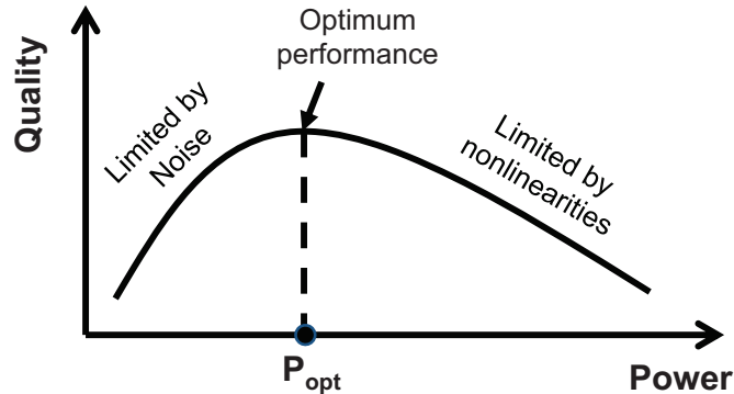
Figure 2.37: Qualitative curve of system quality (or equivalently system reach) in optical telecommunication systems as a function of the injected power per span.
