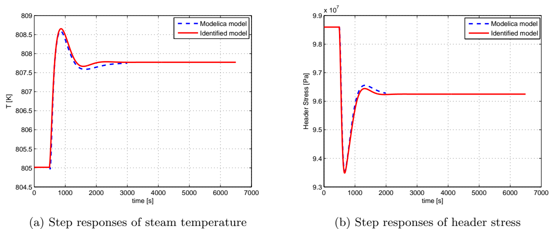
Figure C.1: Comparison between the Modelica and identified model responses at 75%
