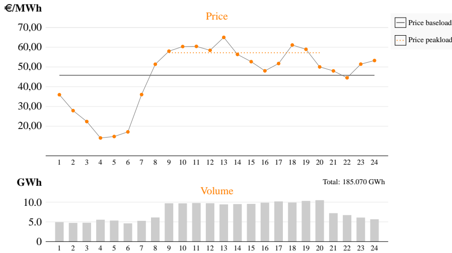
Figure 2.16: Electricity evolution during a day in France (source www.epexspot.com )
