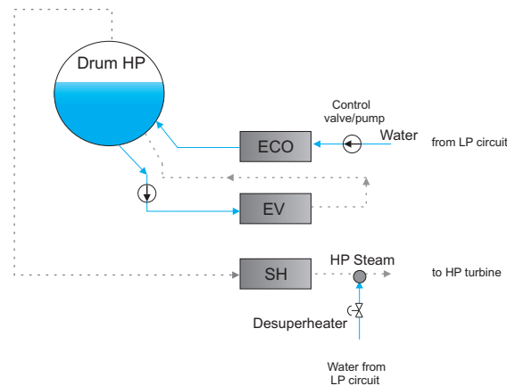
Figure 2.8: HP circuit
