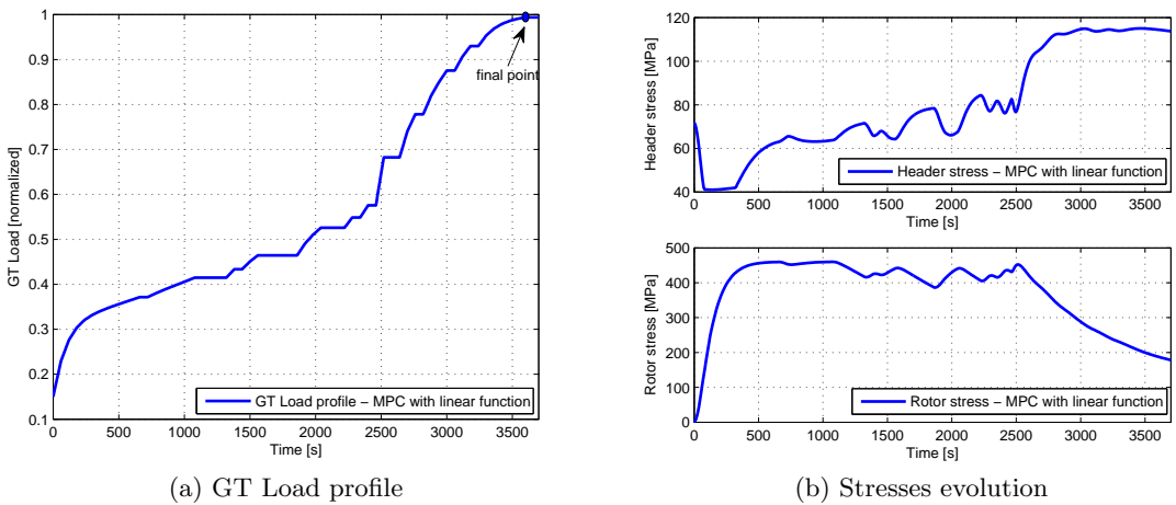
Figure 6.7: MPC GT load profile with linear function. Case study for T_s = 60 s and T_p = 3 * T_s
