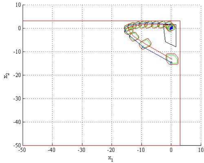
Figure 5.8: Tube trajectory of the closed-loop system fulfilling the state constraints
