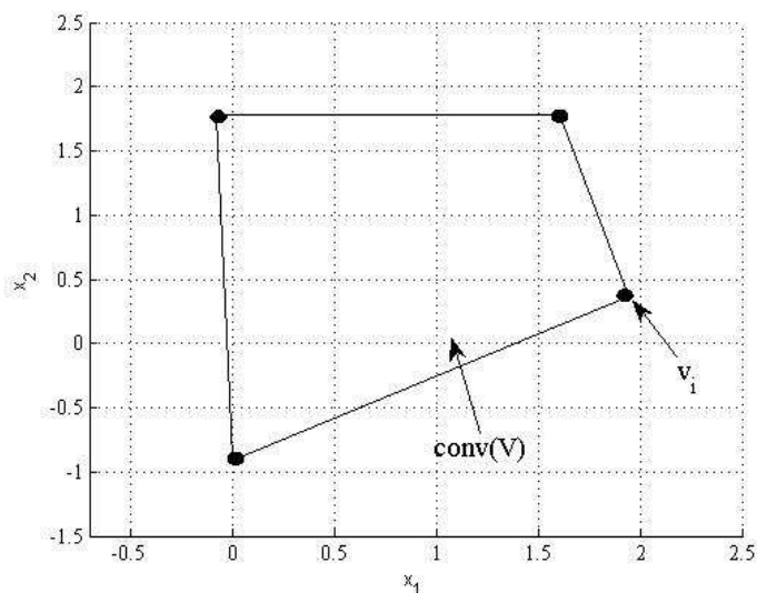
Figure 3.5: V -representation of polytope
