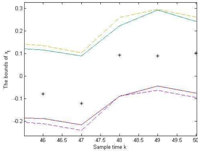
Figure 4.13: Zoom of the guaranteed bound of x_1 obtained by different methods (Example 4.2)
