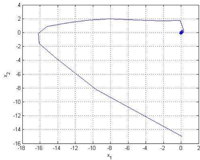
Figure 5.9: Closed-loop response of the system
