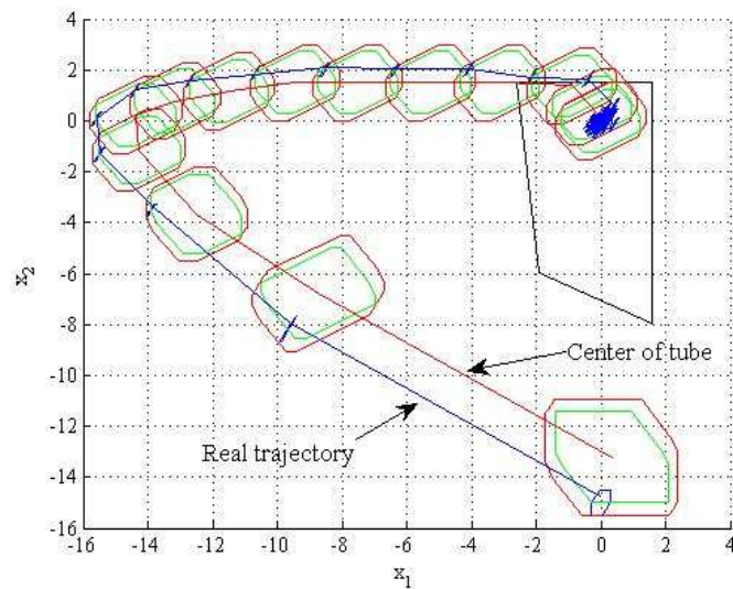
Figure 5.7: Tube trajectory of the closed-loop system
