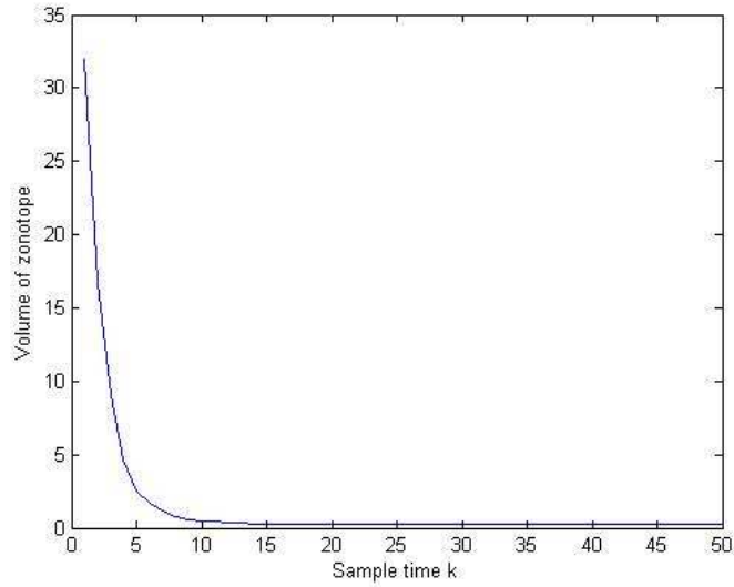
Figure 4.31: Evolution of the volume of the guaranteed state estimation obtained by PMI-based approach
