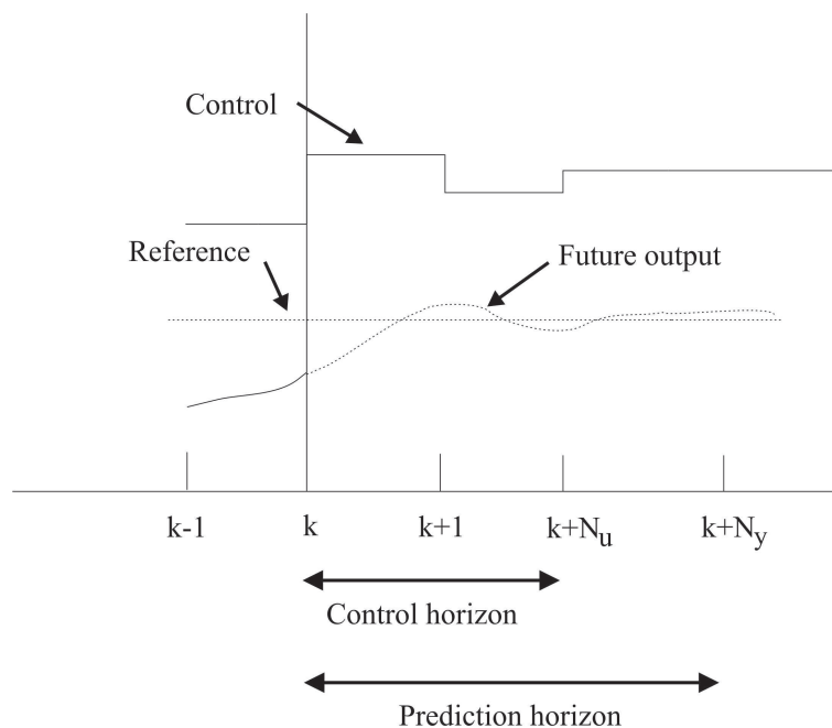
Figure 5.1: Strategy of Model Predictive Control
