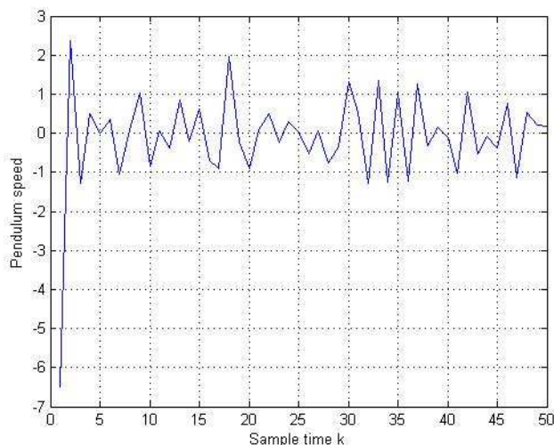
Figure 6.8: Pendulum speed obtained by the open-loop MPC
