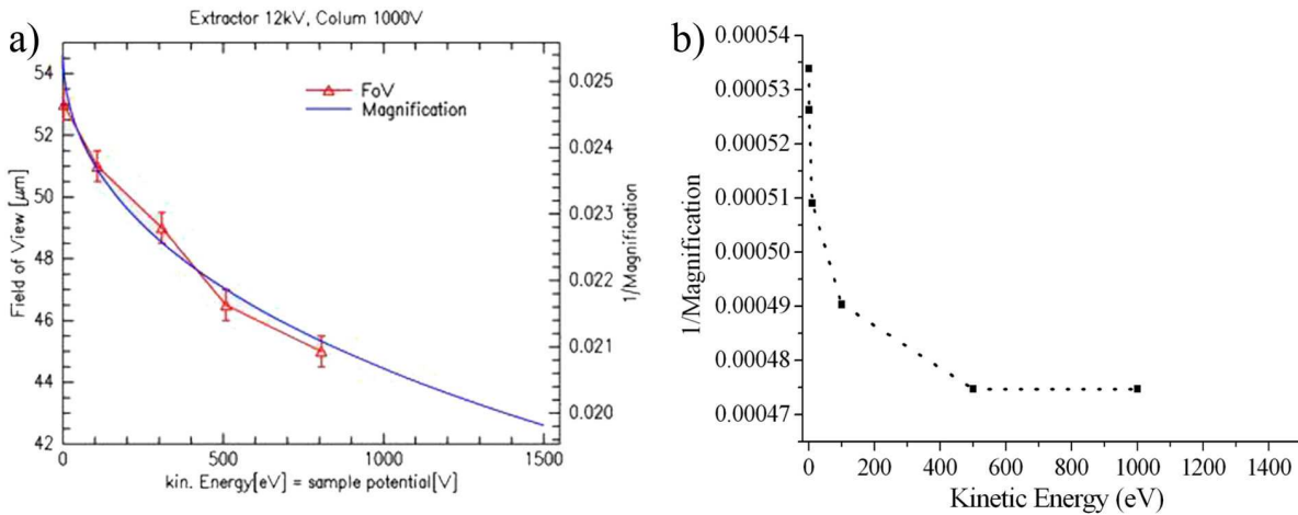
Figure 5.21: Magnification behavior of the PEEM column: a) NanoESCA real case, b) PEEM simplified SIMION case. The scale in y -coordinates in b) is different than a) due to simplifications, but the behavior is the same.
