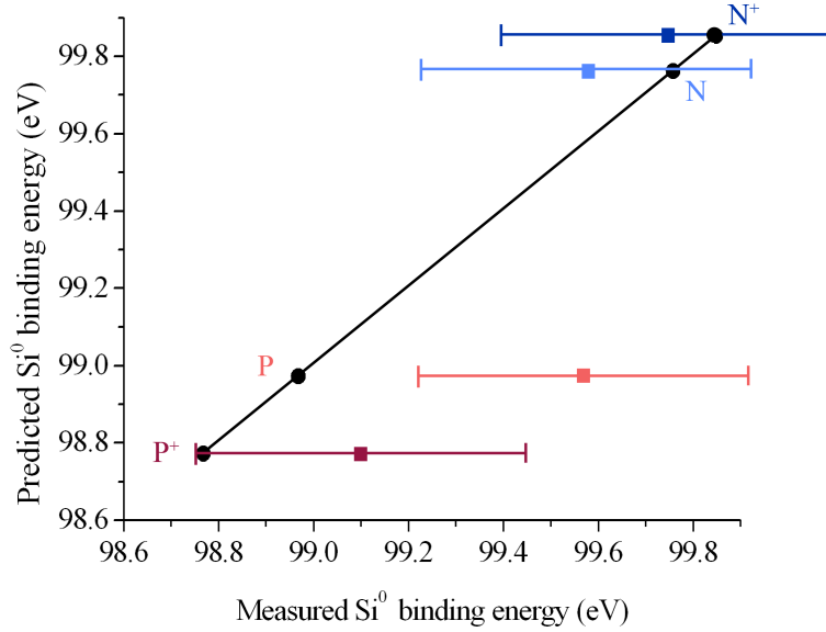
Figure 3.23: Si^0 binding energy measurements for different doping types, and comparison with predicted values from doping in flat band conditions.
