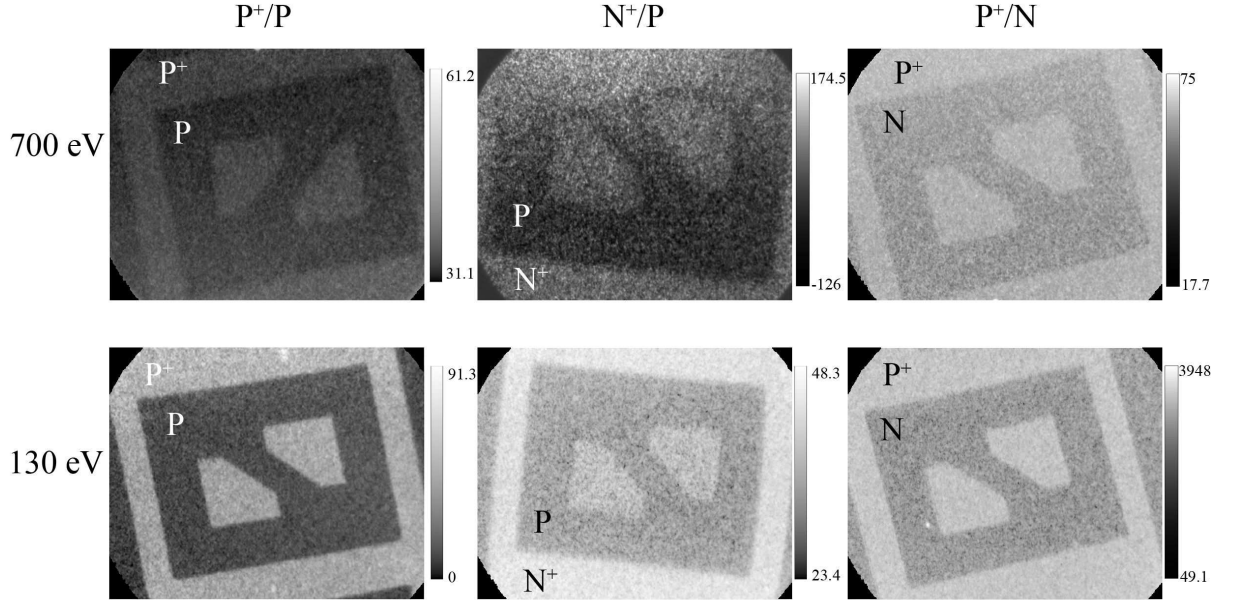
Figure 4.9: Energy-filtered XPEEM images of the integrated \text{Si}^0 intensity for different excitation energies for \text{P}^+/\text{P} , \text{N}^+/\text{P} and \text{P}^+/\text{N} samples (energy range: 97 eV to 101.5 eV). At 700 eV, the higher Si 2p kinetic energy yields to a smaller field of view.
