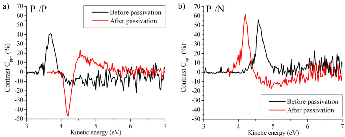
Figure 5.3: Contrast dependence with the sample surface state and kinetic energy for a) N^+/P and b) P^+/N .
