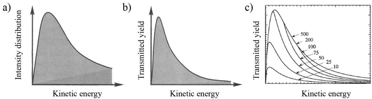
Figure 2.11: SE spectrum before a) and after b) passing through a PEEM column [91, 95]. c) Energy distribution of electrons transmitted through a PEEM, using apertures of different diameters (in \mu\text{m} ) [180].
