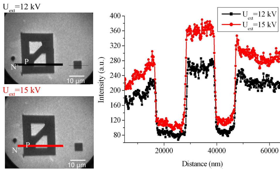
Figure 5.32: Intensity profile of a pn junction taken at threshold ((E - E_F) = 4.75 \text{ eV}) for two extractor voltages: 12 kV (black) and 15 kV (red).
