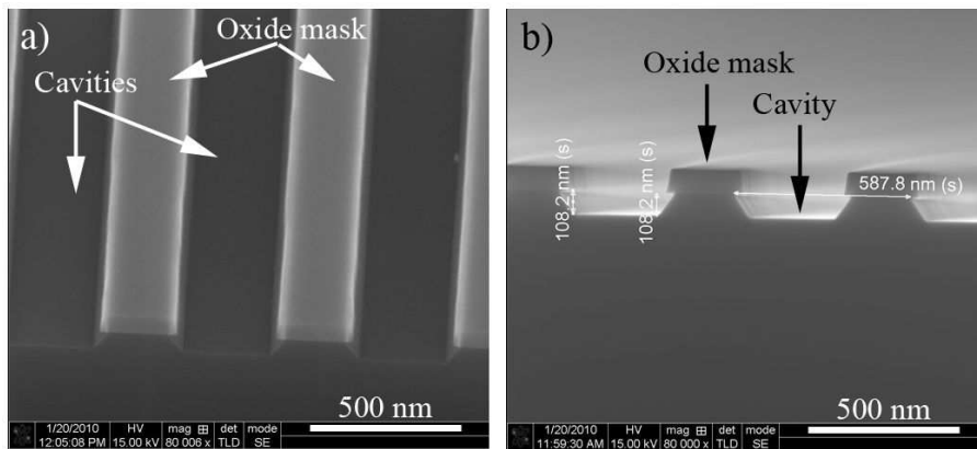
Figure 3.8: SEM images of cross-sectioned silicon chip after HCl recess: view at a) 45^\circ and b) normal observation.
