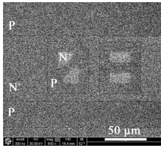
Figure 5.14: SE image of N^+/P acquired with FIB.
