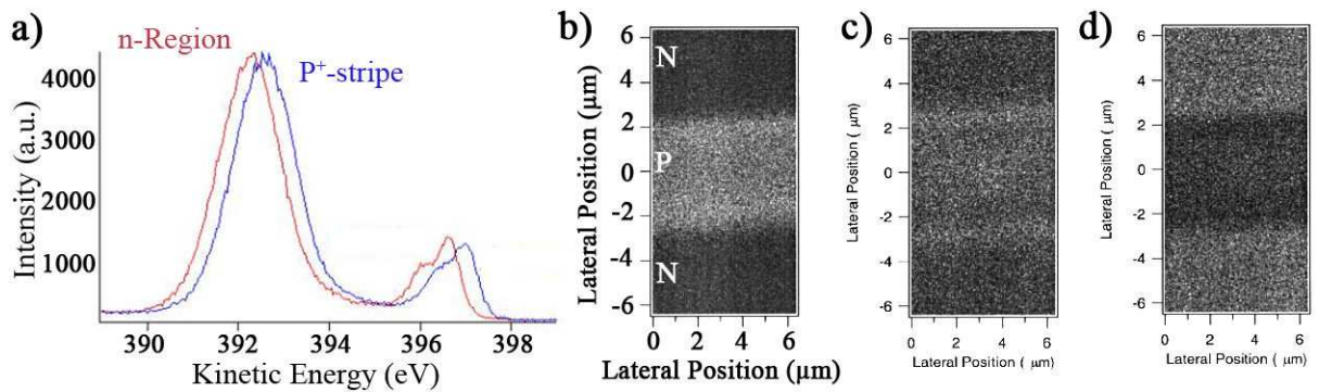
Figure 1.12: a) Scanned Si 2p SPEM intensity maps showing energy dependent contrast across a silicon p-stripe, at electron energies of b) 397.22 eV, c) 396.98 eV, and d) 396.82 eV. Field of view (FoV) is (6.4 \pm 12.8) \mu\text{m} [94].
