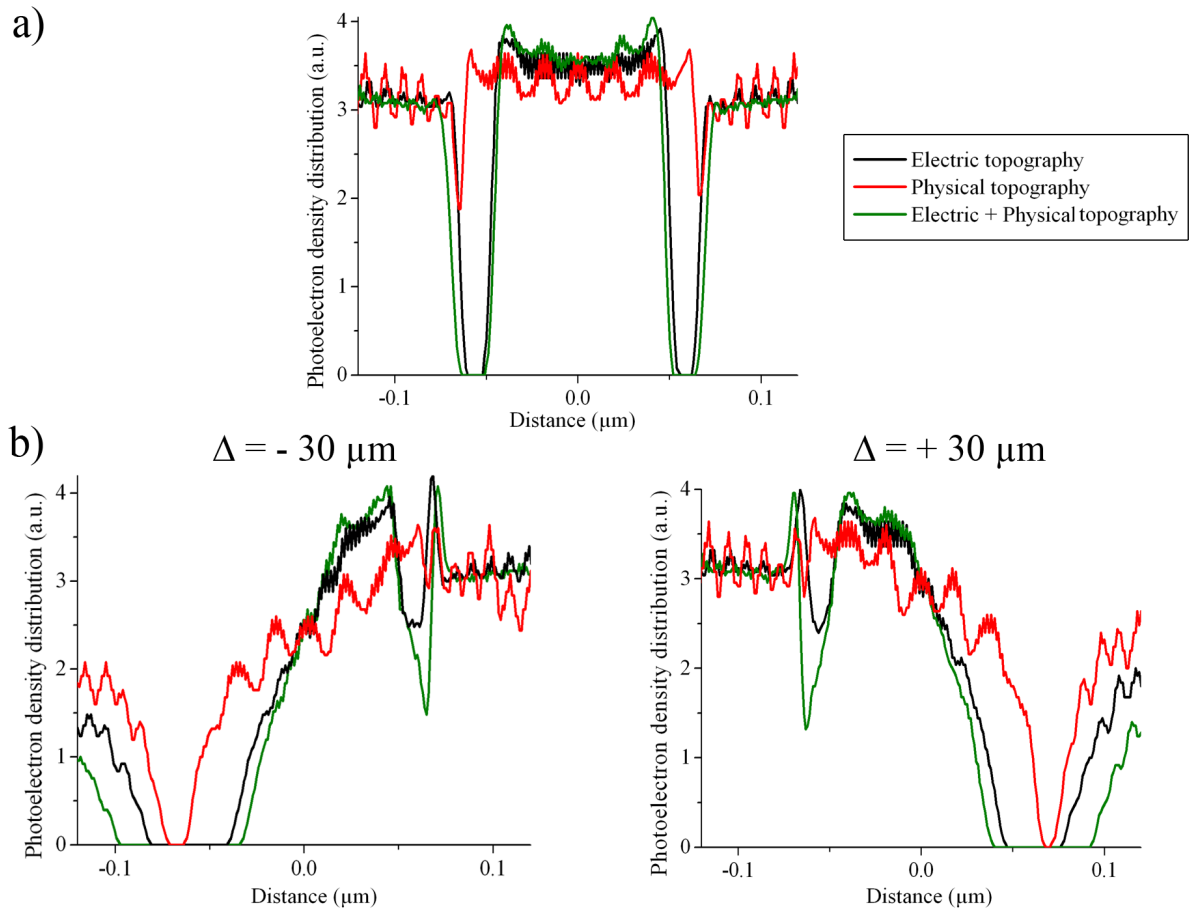
Figure 5.44: Influence of topography on PEEM imaging, for cases of electric topography alone, lateral one alone, and the both combined with: a) CA centered and b) CA shifted by \Delta = \pm 30 \mu\text{m} .
