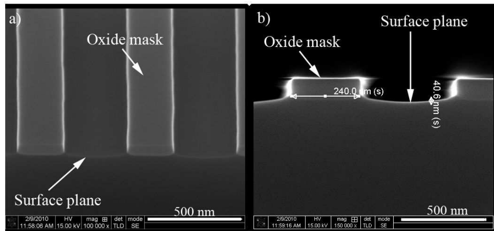
Figure 3.10: SEM images of cross-sectioned silicon chip after localized boron epitaxy at a) 45^\circ and b) normal observation.
