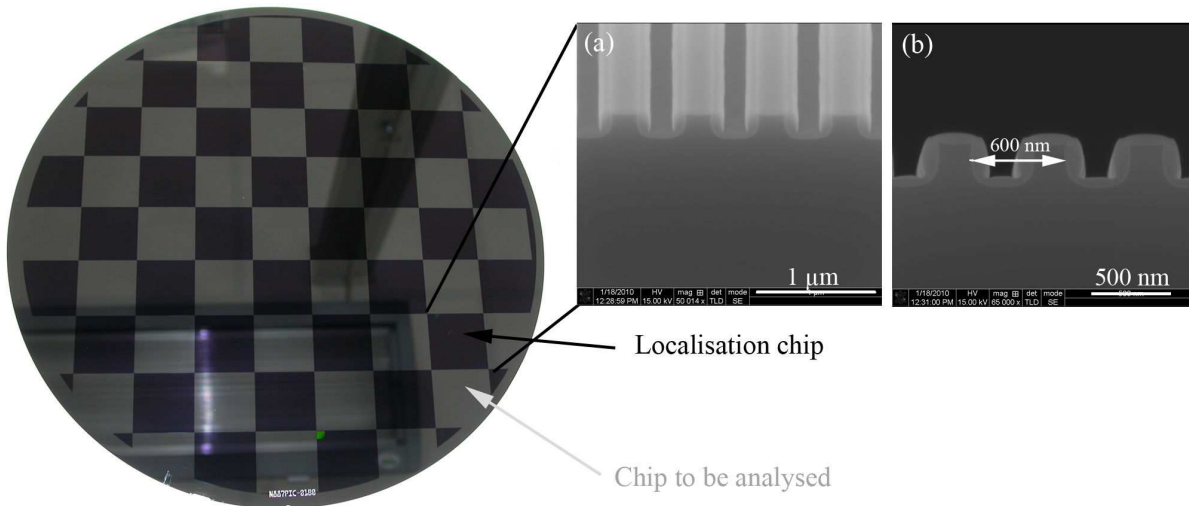
Figure 3.7: Optical image of a wafer. Onset: SEM images of one cross-sectioned silicon chip used for localisation: one clearly sees the oxide coverage in light gray on a) 45^\circ view, and b) normal observation. S=L=300 nm.
