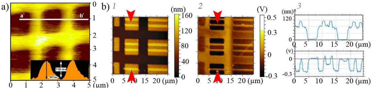
Figure 1.6: a) Surface potential image of a pn junction array measured by KFM [46]. b) The topography 1- and surface potential 2- images of Static Random Access Memory (SRAM). The cross-section profiles along the directions indicated with red arrows in 1- and 2- are shown in the top and bottom parts of 3- [47].
