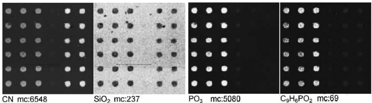
Figure 1.2: Negative ToF-SIMS images of a Si wafer PNA/DNA biosensor chip. (25 keV Bi 3+ , field of view (1500 × 1500) nm 2 . Light gray corresponds to high intensity [9].
