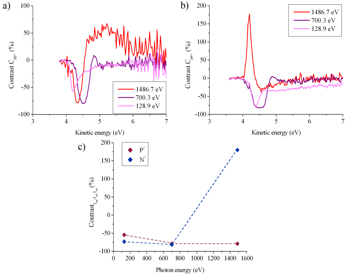
Figure 5.5: Contrast comparison between a) \text{P}^+ and b) \text{N}^+ relatively to P bulk taken at threshold for three photon energies. c) Maximum contrast measured for several photon energies for \text{P}^+ and \text{N}^+ doping type.
