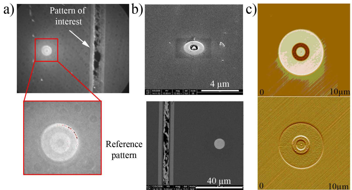
Figure 2.28: W pattern realized by FIB and observed by: a) Energy-Filtered PEEM, b) SEM, c) AFM.
