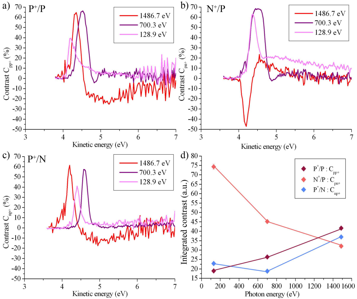
Figure 5.4: Contrast taken at threshold for three photon energies for a) P + /P , b) N + /P and c) P + /N. d) Contrast evolution of the integrated intensity between 3 eV and 6 eV, with the photon energy. The uncertainty is estimated to be \pm 2\% .
