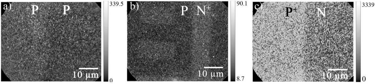
Figure 4.6: Energy-filtered XPEEM images at the Si^0 core-level at 1486.7 eV photon energy (energy range: 98 eV to 101.5 eV).
