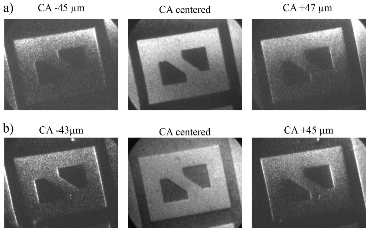
Figure 5.46: Dark field imaging on passivated P^+/P sample at threshold with a photon source of a) 700.3 eV and b) 128.9 eV.
