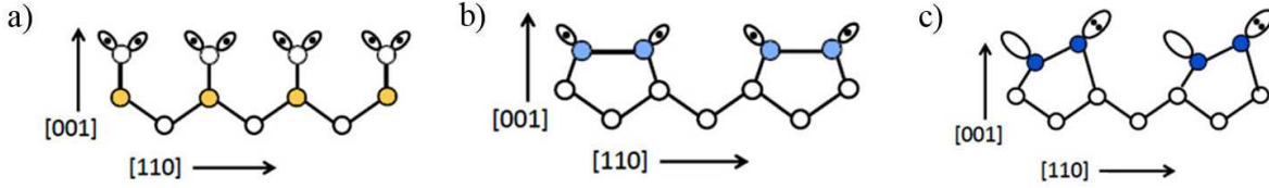
Figure 3.22: Sections through a) the Si second layer, b) the Si (2x1) symmetric dimer surface and c) the (2x1) asymmetric dimer surface. The dimer bond is in the plane of the paper, the dimer rows running perpendicularly out of the plane of the paper.
