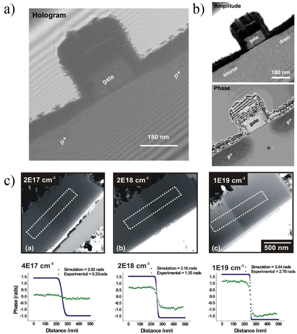
Figure 1.8: a) Hologram of a 0.18 \mu\text{m} p-MOS transistor structure. b) Reconstructed amplitude and phase image of the transistor [60]. c) Top images represent phase images of 400 \text{ nm} -thick-specimen for each of the pn junctions with different doping, and prepared by conventional FIB milling. Bottom images show the experimental phase profile extracted from the white rectangles, compared to the theoretical step in phase for perfect bulk-like specimens [66].
