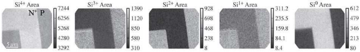
Figure 2.27: Silicon sub-oxide peak area maps obtained from best fits to the Si 2p spectra generated from the highly n -doped zone on p -doped silicon bulk [222].
