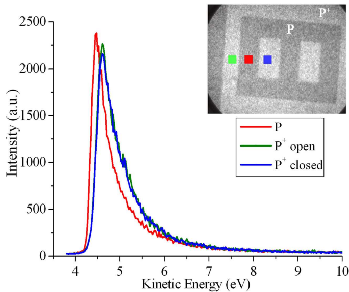
Figure 5.1: Image XPEEM of P^+/P sample taken at threshold. The photon energy is 700.3 eV.
