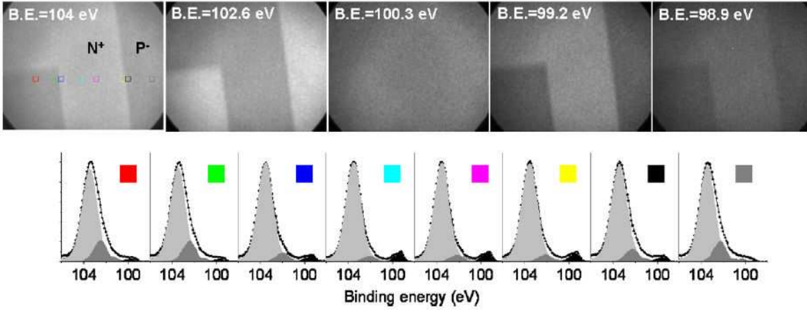
Figure 1.13: Top: selected XPEEM images from the energy filtered image series across the Si 2p core level on sample N + /P. Bottom: local Si 2p core level spectra and best least squares fits: the Si 4+ component due to the native SiO 2 oxide is in light gray, the sub-oxide components gray and the Si 0 substrate component black. FoV is 25 μm [101].
