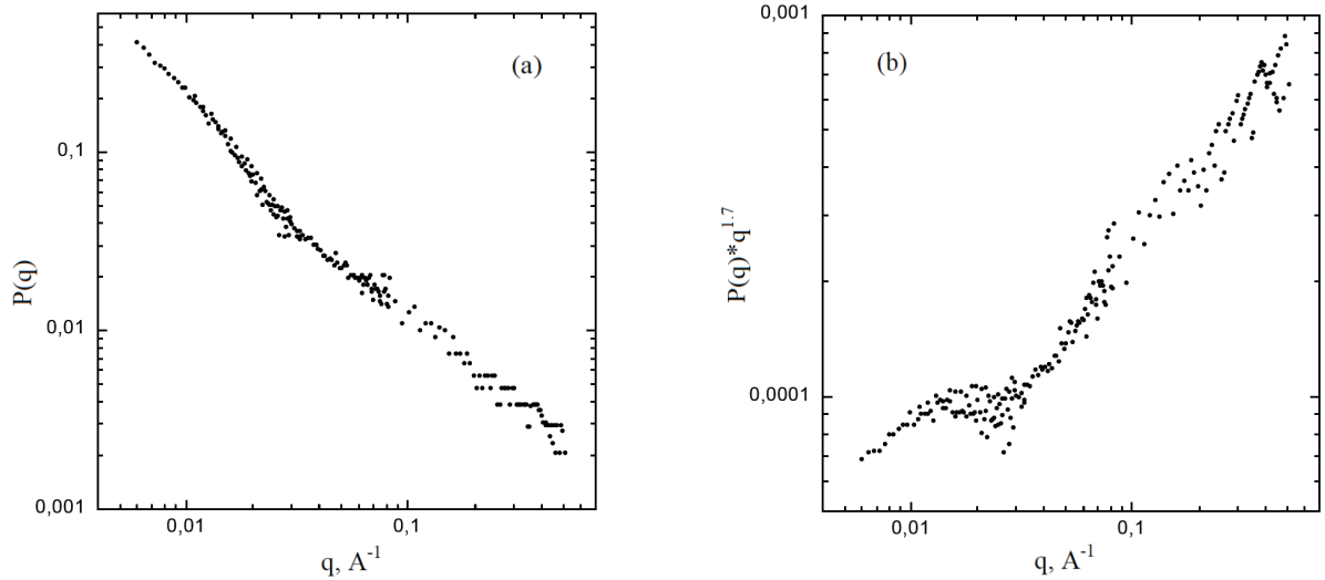
Figure 8. PSSH aqueous solutions studied by SANS at ZAC condition: (a) P(q) vs. q ; (b) P(q)*q^{1.7} vs. q .
