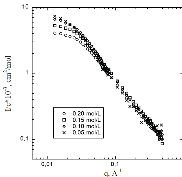
Figure 15. Scattering profile of PSS ( N = 300 ) solutions in IL1 at 80°C obtained by SANS.
