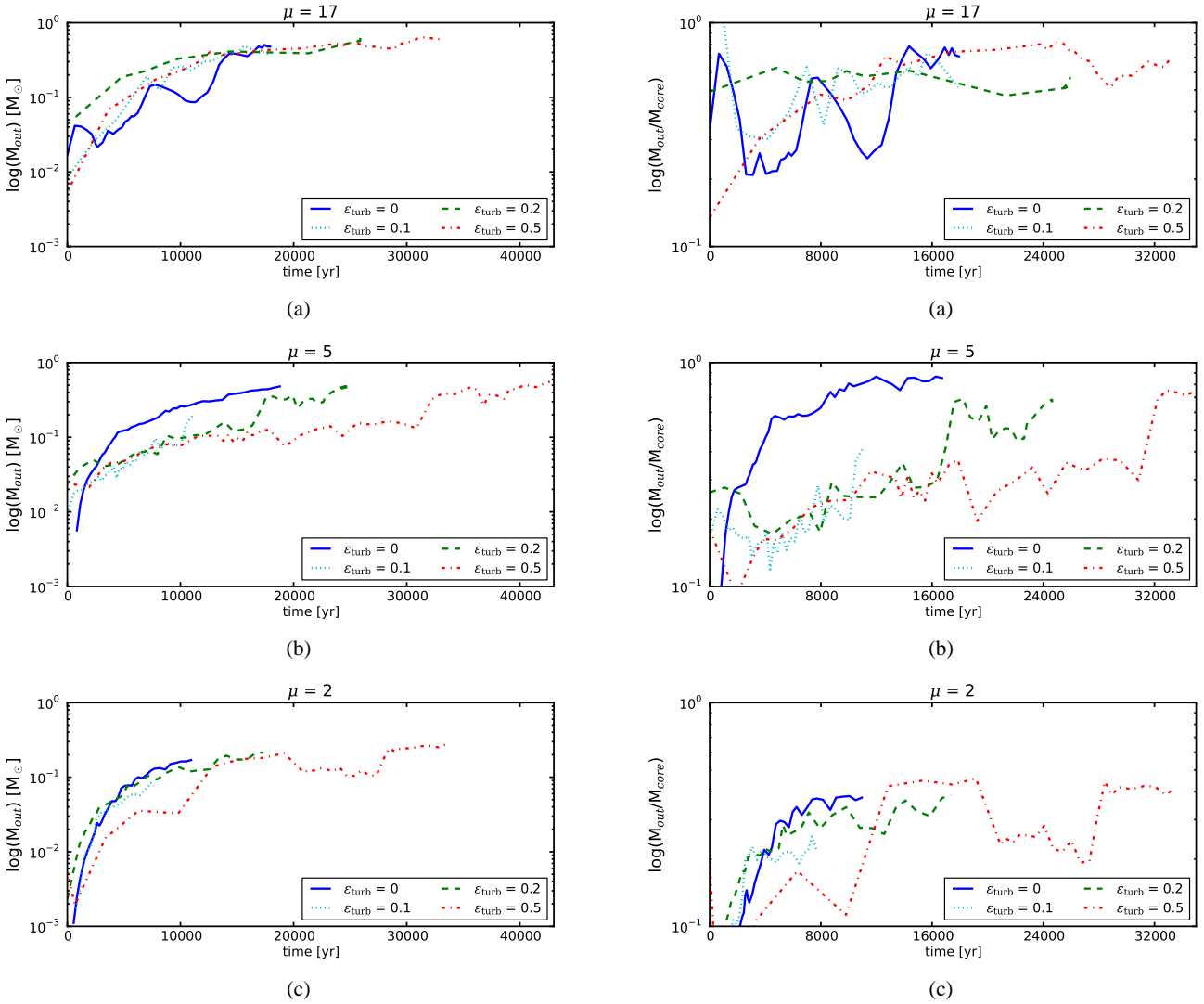
Figure 11. Total mass in the outflows for \mu = 17, 5, and 2 , without turbulence, with \epsilon_{\text{turb}} = 0.1, 0.2, and 0.5 .
