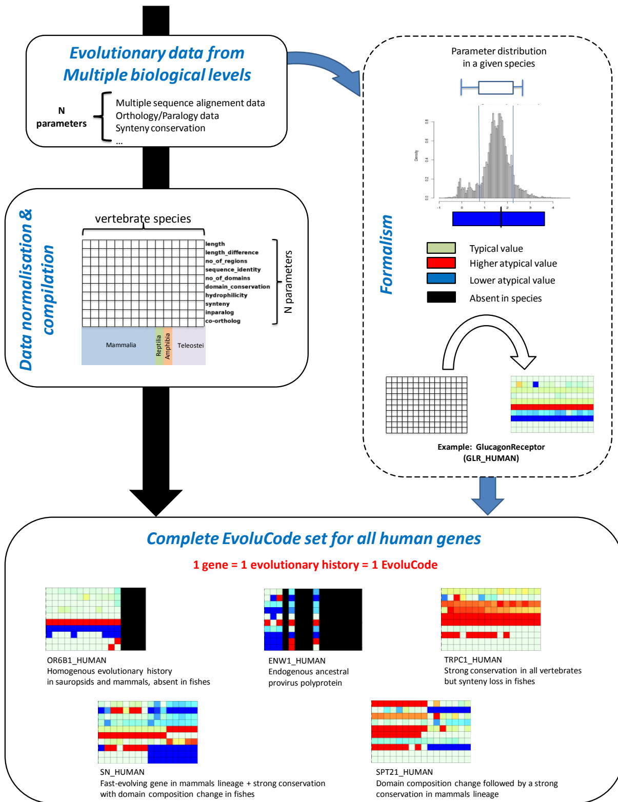
Figure 8-4: Overview of the EvuCode construction process. Different evolutionary parameters are compiled from several sources and organised in the EvuCode framework. A parallel process statistically describes the variation of these parameters when comparing the vertebrate’s parameter states compared to the human reference. The statistical model is used to create the EvuCode formalism that allows a direct human visualization of variation profiles corresponding to different gene evolutionary histories.
