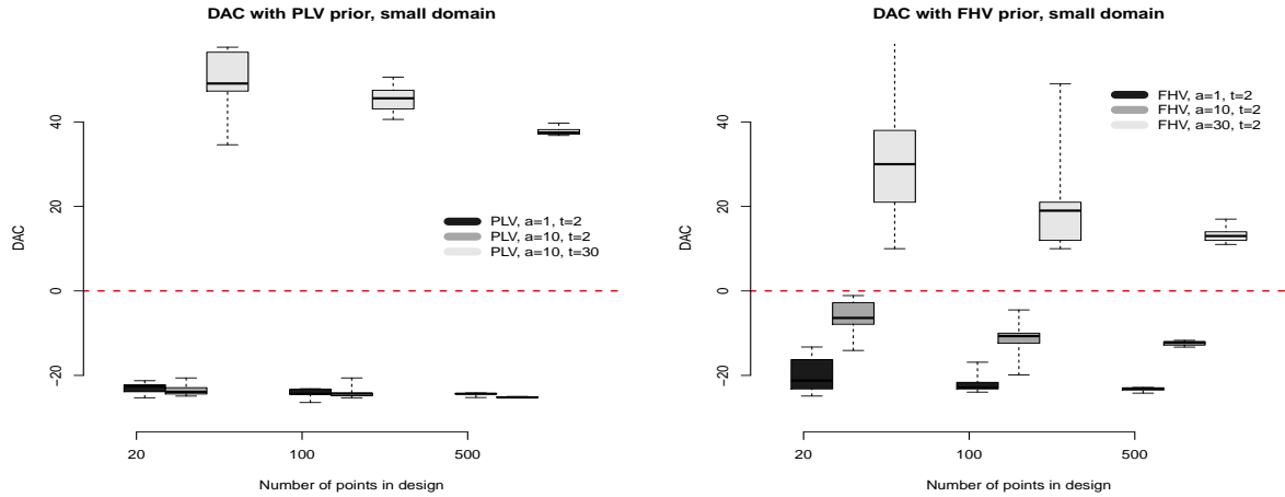
Figure IV.7: \widehat{DAC} with PLV and FHV priors for the small domain \Omega_1 and different values of the hyperparameters a and t
