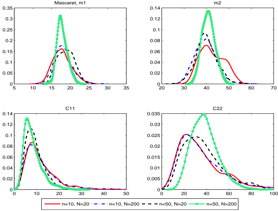
Figure VI.8: Posterior distributions of \theta with perfect prior, the sample size n = 10, 50 and maximin -LHDs D_{20}, D_{200}
