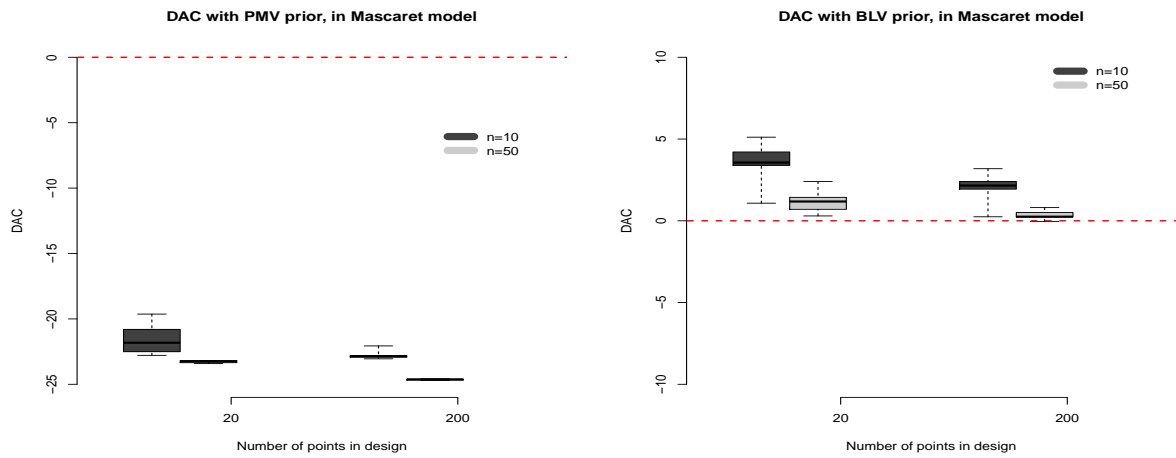
Figure VI.16: \widehat{DAC} with PMV and BLV priors, based on n = 10, 50 observations and two maximin -LHDs D_{20} and D_{200} , in the MASCARET code
