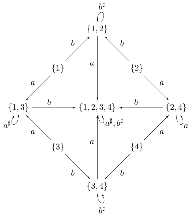
Figure 6.10: The support graph of the automaton depicted in Fig 6.9.
