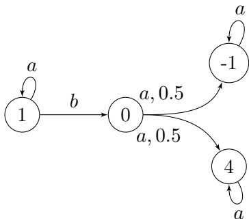
Figure 3.5: Markov decision process where the mean-payoff and positive-average objectives have different optimal strategies
