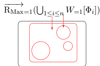
Figure 3.4: Solving disjunction of tail objectives
