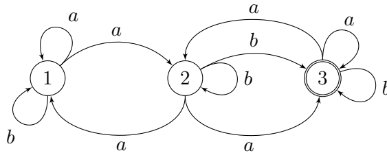
Figure 6.11: This automaton has value 1 and is not \sharp -acyclic .
