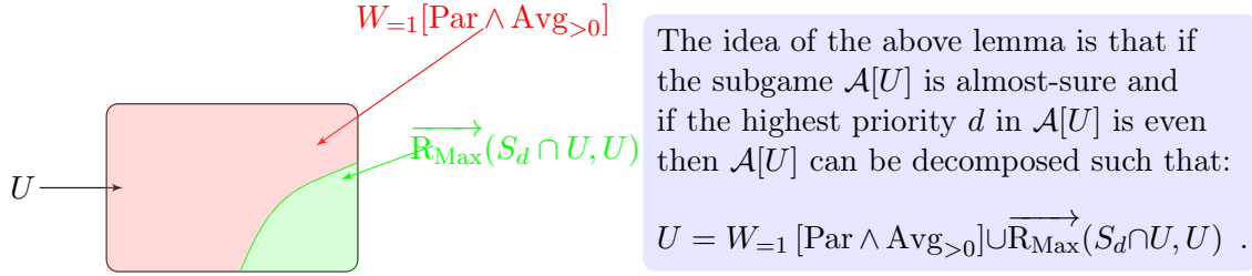
Figure 5.1: Decomposition of \mathcal{A}[U] when the highest priority is even
