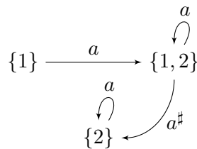
Figure 6.8: The support graph of the automaton depicted in Fig 6.7
