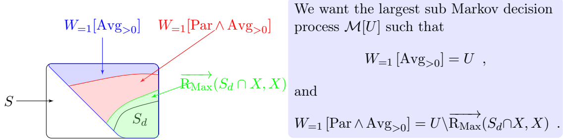
Figure 4.1: Construction of the almost-sure region when the highest priority is even.
