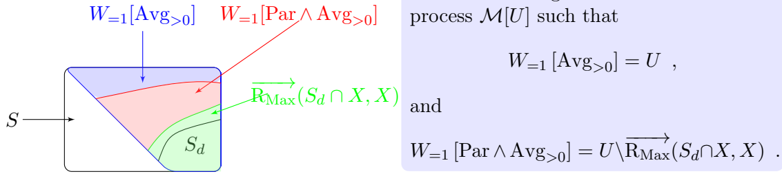
Figure 4.1: Construction of the almost-sure region when the highest priority is even.
