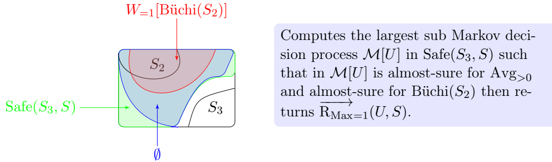
Figure 4.3: Construction of the almost-sure region W_{=1}[\Phi_d] .
