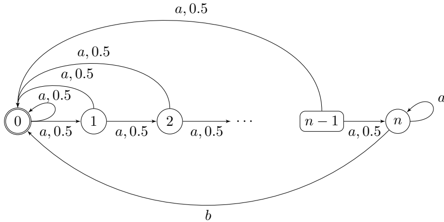
Figure 4.6: Max needs a memory of size exponential to achieve almost-surely the objective \text{Par} \wedge \text{Avg}_{>0} .
