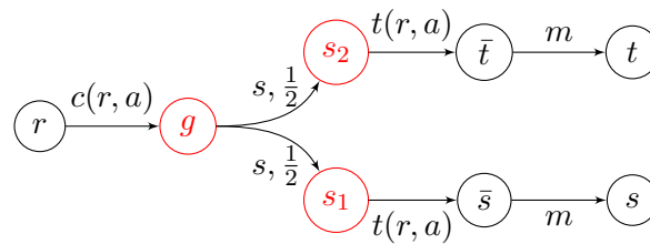
Figure 6.4: Gadget for a probabilistic transition
