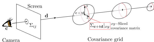
Figure 5.19 – We accumulate spatial covariance matrices from the covariance grid by ray marching. In each voxel, we slice the covariance of the fluence's spectrum and add the eye path attenuation and occlusion to it. The resulting 2D matrices are averaged using intensity weights.
