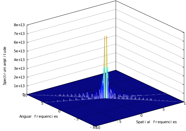
Figure 3.16 – The non-planar occluder approximation is a wedge function. It explains why the planar slice approximation of occluders works [108, 51, 50]. Furthermore, we only need to provide the first and last slice of the occluder to obtain a decent estimate of the occlusion. For this figure, we used t_{min} = 50\text{cm} and t_{max} = 1\text{m} . We used d = 0 to have a real valued spectrum.
