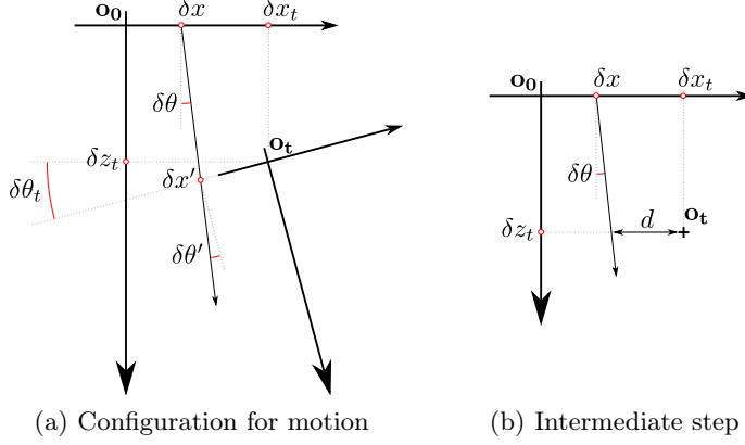
Figure 3.33 – The effect of motion on positions and angles is illustrated here. We study 2D coordinates (\delta x, \delta\theta) and its transformation after a unit time motion : (\delta x', \delta\theta') . The tangential motion of space \mathbf{o}_t with respect to space \mathbf{o}_0 is \delta x_t . The non-tangential motion is \delta z_t and the angular motion is \delta\theta_t (a). To obtain the value \delta x' we need an intermediate step and compute the distance of the photon at position (\delta x, \delta\theta) after a travel of \delta z_t meters along the Z axis with respect to the time changing center \mathbf{o}_t (b).
