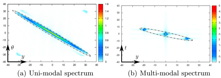
Figure 4.13 – Our analysis is uni-modal. We obtain the information about the complete spectrum using a covariance analysis for example (a). But a spectrum can be composed of distinct frequency elements on which a multi-modal analysis could be beneficial (b). In the case presented here, there is a low frequency component around the DC and an anisotropic high frequency component with a close to Gabor type.
