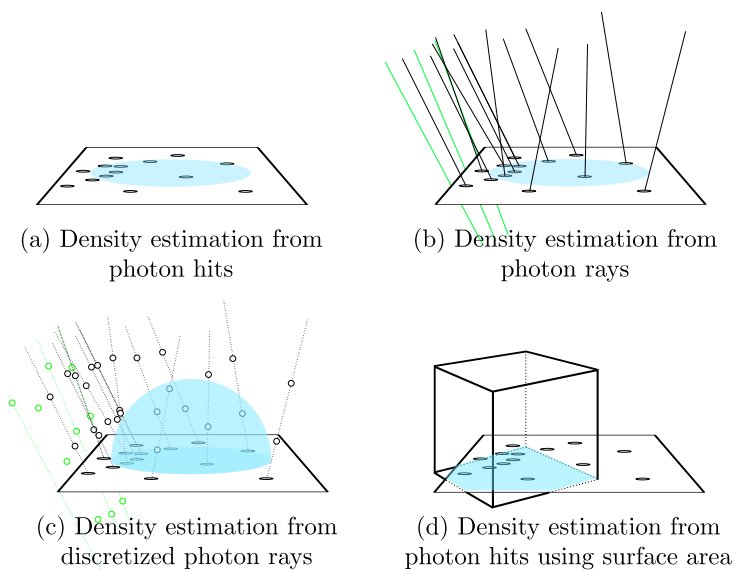
Figure 2.5 – Here we review the different density estimators proposed for radiance estimation on surfaces. Jensen [92] used photon hits in a k -nearest fashion (a). Lastra et al. [109] evaluated the light-field radiance on a planar disc using photon rays (b). Zinke and Weber [191] discretized photon rays to accelerate the density evaluation (c). Hey and Purgathofer [79] used the surfaces inside a cube perform the integration. Rays in green are not intersecting the surface but also contribute to the estimator.
