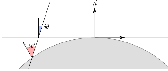
Figure 3.21 – The curvature operator flattens the input local light-field against the local surface. While the positions are approximately equal (to first order), the angles are modified with respect to their positions.
