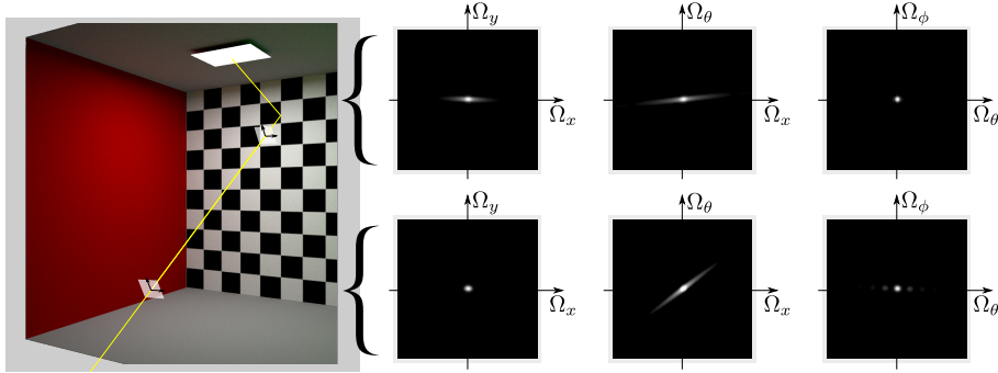
Figure 3.11 – We display slices of the Fourier amplitude. The shear effect is visible on the spatio-angular slice. Indirect effects of the shear are visible in the spatial slice as a part of the energy goes to the angular domain.
