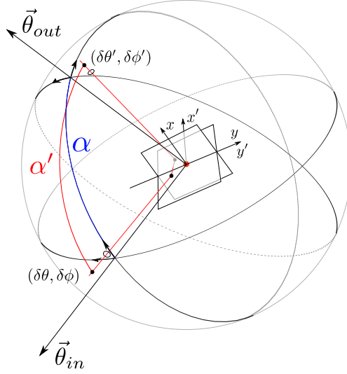
Figure 3.24 – If the parametrization of the BRDF, or BTDF, follows the equatorial plane, we can use additive notations of angles. To first order, the angular difference is \alpha' \simeq \alpha - (\delta\theta_1 - \delta\theta_2)
