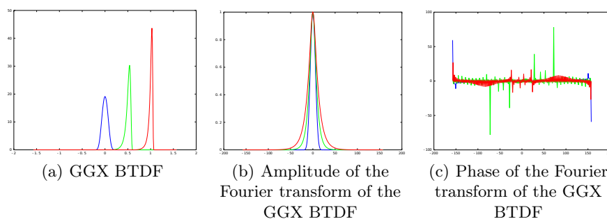
Figure 3.27 – GGX BTDFs are not isotropic for grazing angles (a), but the amplitude of their Fourier transform is (b). The non-symmetrical information is stored in the phase (c). We approximate the Fourier spectrum of GGX BTDFs by Gaussians which standard deviation correspond to the inverse roughness, much like de Rousiers et al. [39]. We used a glass index of n = 1.1 , the incoming angles are 0 , \frac{\pi}{6} , and \frac{\pi}{3}
