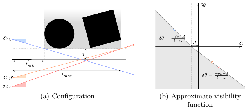
Figure 3.14 – We model the correlation between space and angles using the following configuration (a). Given a set of occluders, we analyse the resulting occlusion bounding box. Close to Egan et al.’s [51] analysis, we define the minimum and maximum distance of occlusion and look at the resulting visibility function. We obtain a piece-wise rotated half-plane ocluder (b).
